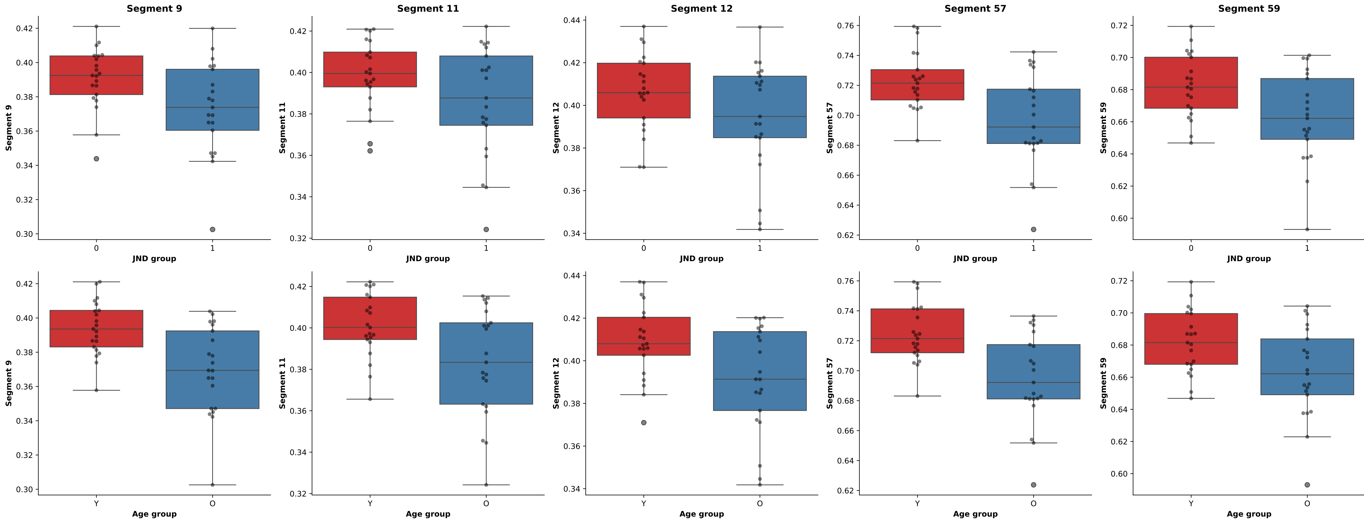
Boxplot of selected features groups for CC 4
