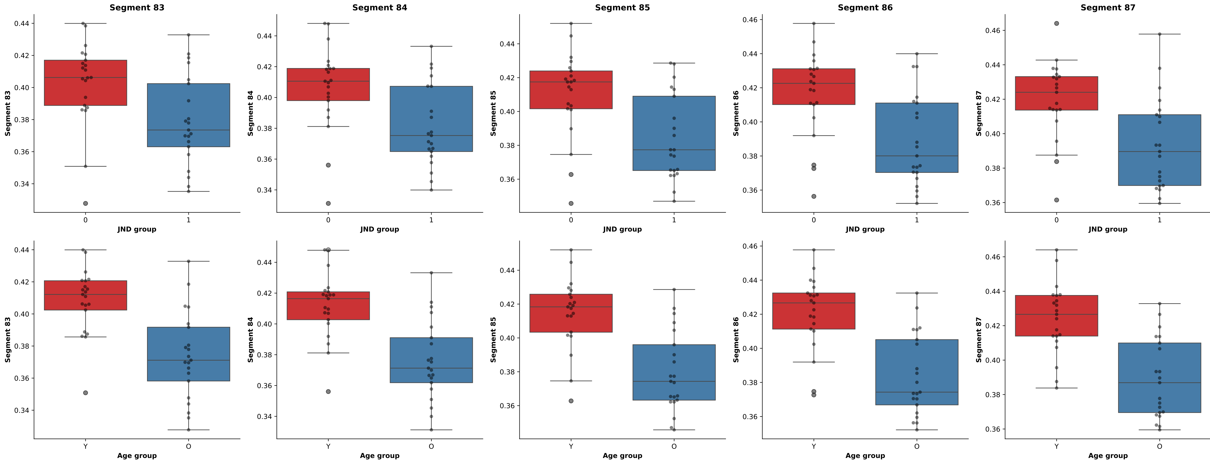
Boxplot of selected features groups for CC 5
