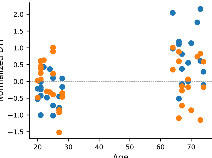
Age vs DTI (CC1, segment 10)
