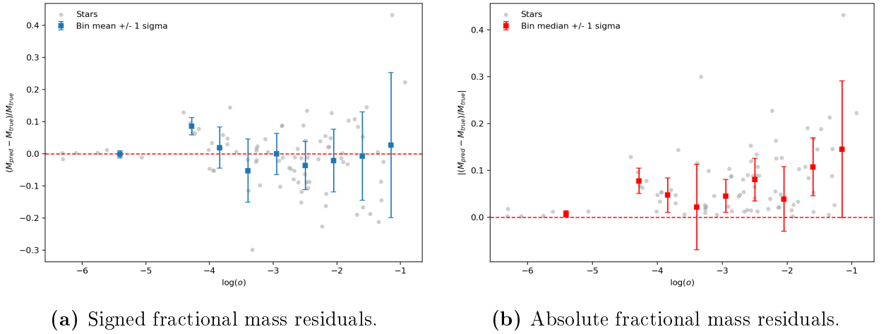
Figure 7: Dependence of the BHS mass residuals on stellar oblateness o , as defined in Equation 4, for the selected eclipsing-binary sample. The model uses T_{\text{eff}} , L , \log g and [\text{Fe}/\text{H}] as input parameters. Grey points correspond to individual eclipsing-binary components, and the blue and red squares show binned means and medians with 1\sigma scatter. The sample contains n = 85 stars.
