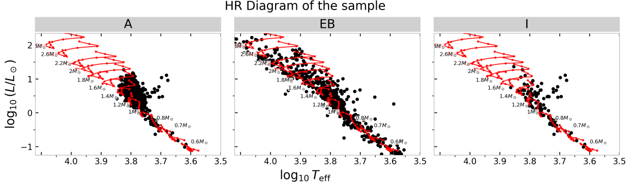
Figure 3: HR diagram of the 767 stars in the final sample. The red curves are theoretical evolutionary tracks of different masses obtained with PARSEC (Bressan et al., 2012). The sample is divided by the main method used to study each star: asteroseismology, eclipsing binaries and interferometry.
