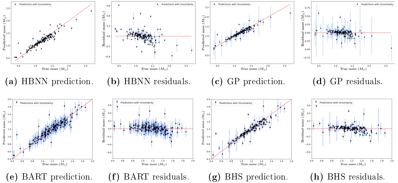
Figure 5: Holdout-test performance of the HBNN, GP, BART and BHS mass models trained with T_{\text{eff}} , L and [\text{Fe}/\text{H}] . For each model, the prediction panel shows M_{\text{pred}} as a function of M_{\text{true}} , while the residual panel shows M_{\text{pred}} - M_{\text{true}} as a function of M_{\text{true}} . Vertical error bars represent the predictive uncertainty returned by each model. The GP and BHS panels are restricted to the stars below the 95th percentile of predicted mass uncertainty in order to keep the main population visually readable. The full calibration sample contains n = 767 stars, with 20% reserved for the holdout test.
