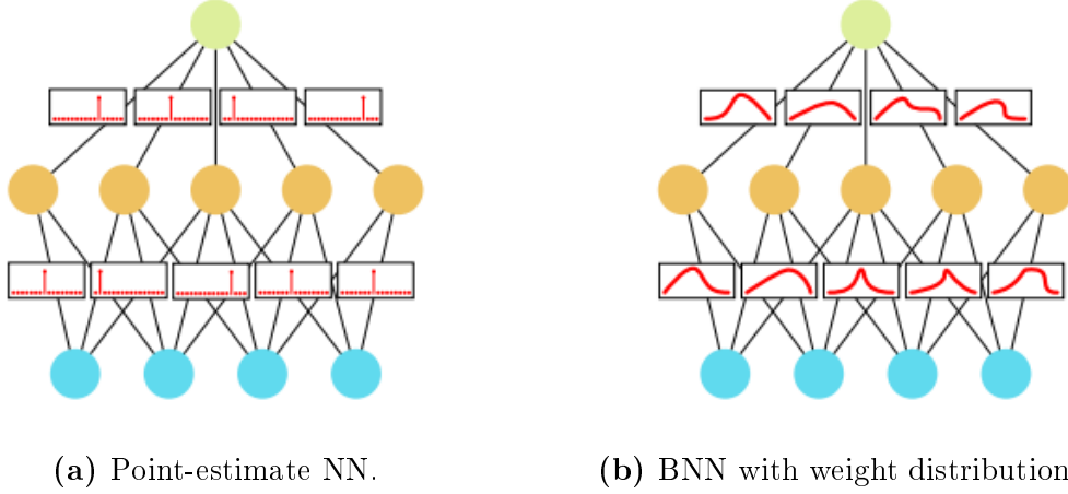
Figure 4: Comparison between neural-network formulations. Figure 3a shows a standard network, in which the weights and biases are fixed after training. Figure 3b shows the Bayesian formulation used in this work, where probability distributions are assigned to the weights and biases. Adapted from (?).
