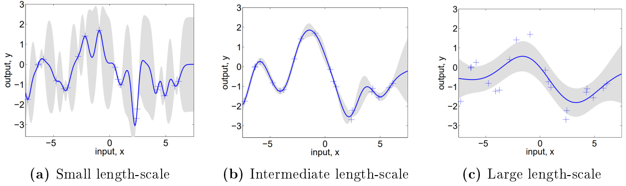
Figure 3: Example of Gaussian Process posterior predictions obtained for the same training points using different length-scales. The shaded regions show the corresponding predictive uncertainty. Reproduced from Figure 2.5 of ?.
