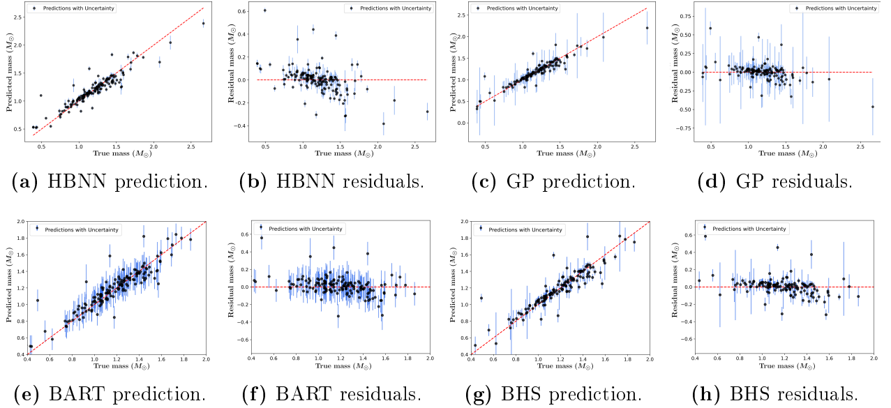
Figure 7: Holdout-test performance of the HBNN, GP, BART and BHS mass models trained with T_{\text{eff}} , L and [\text{Fe}/\text{H}] . For each model, the prediction panel shows M_{\text{pred}} as a function of M_{\text{true}} , while the residual panel shows M_{\text{pred}} - M_{\text{true}} as a function of M_{\text{true}} . Vertical error bars represent the predictive uncertainty returned by each model. The GP and BHS panels are restricted to the stars below the 90th percentile of predicted mass uncertainty in order to keep the main population visually readable. The full calibration sample contains n = 767 stars, with 20% reserved for the holdout test.
