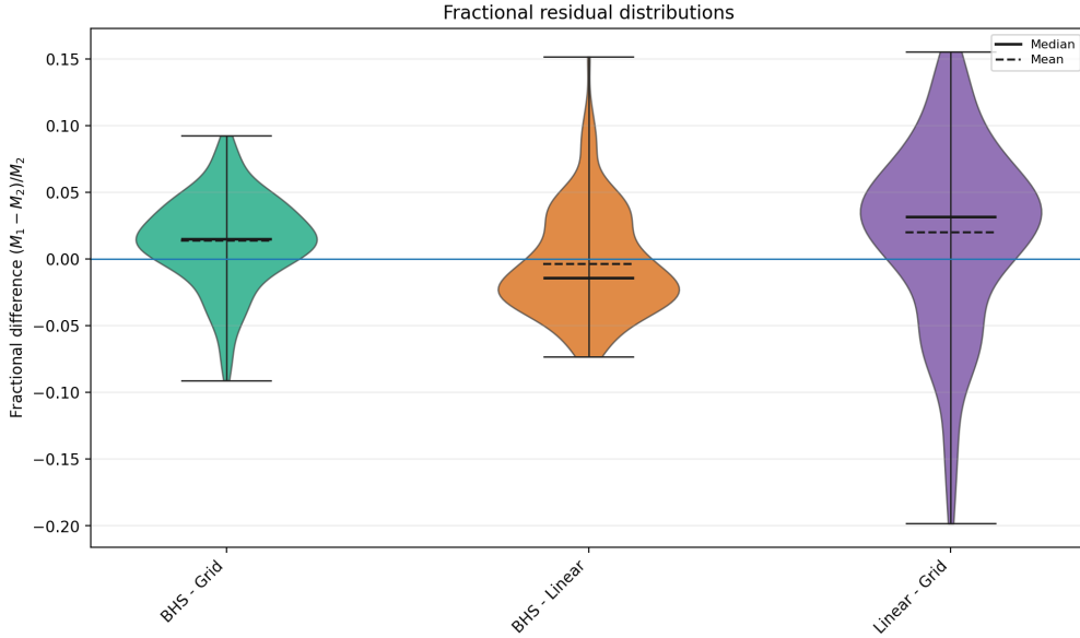
Figure 8: Distributions of fractional mass residuals for the comparison between the Bayesian Hierarchical Stacking predictions and the two reference mass estimates used for the ARIEL sample. The green distribution compares BHS with the stellar-model grid masses provided by the IA-Porto group, while the orange distribution compares BHS with the linear-relation masses from ?. The purple distribution shows the direct comparison between the linear-relation and grid masses. The fractional residuals are defined as (M_1 - M_2)/M_2 , following the order of the two methods shown on the horizontal axis. The sample contains n = 184 stars.
