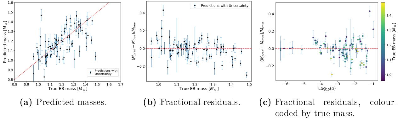
Figure 10: Analysis of BHS residuals for the selected eclipsing-binary sample of 85 stars. The model uses T_{\text{eff}} , L , \log g and [\text{Fe}/\text{H}] as input parameters. The left panel compares predicted and reference EB masses, the central panel shows the corresponding fractional residuals as a function of true mass, and the right panel shows the fractional residuals as a function of stellar oblateness o , colour-coded by true mass. Error bars show the propagated predictive uncertainty, and the dashed red line marks zero residual.
