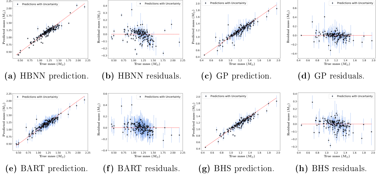
Figure 6: Holdout-test performance of the HBNN, GP, BART and BHS mass models trained with T_{\text{eff}} , \rho and [\text{Fe}/\text{H}] . For each model, the prediction panel shows M_{\text{pred}} as a function of M_{\text{true}} , while the residual panel shows M_{\text{pred}} - M_{\text{true}} as a function of M_{\text{true}} . Vertical error bars represent the predictive uncertainty returned by each model. The GP and BHS panels are restricted to the stars below the 95th percentile of predicted mass uncertainty in order to keep the main population visually readable. The full calibration sample contains n = 767 stars, with 20% reserved for the holdout test.
