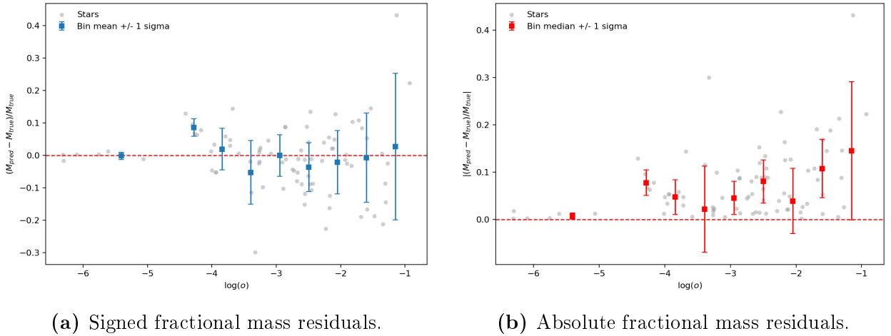
Figure 9: Dependence of the BHS mass residuals on stellar oblateness o , as defined in Equation 3, for the selected eclipsing-binary sample. The model uses T_{\text{eff}} , L , \log g and [\text{Fe}/\text{H}] as input parameters. Grey points correspond to individual eclipsing-binary components, and the blue and red squares show binned means and medians with 1\sigma scatter. The sample contains n = 85 stars.
