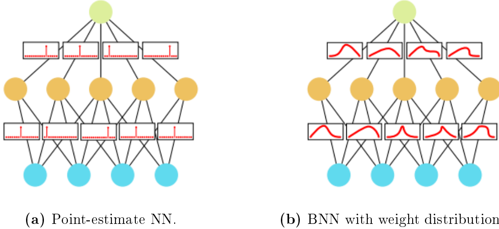
Figure 2: Comparison between neural-network formulations. Figure 2a shows a standard network, in which the weights and biases are fixed after training. Figure 2b shows the Bayesian formulation used in this work, where probability distributions are assigned to the weights and biases. Adapted from (Jospin et al., 2022).
