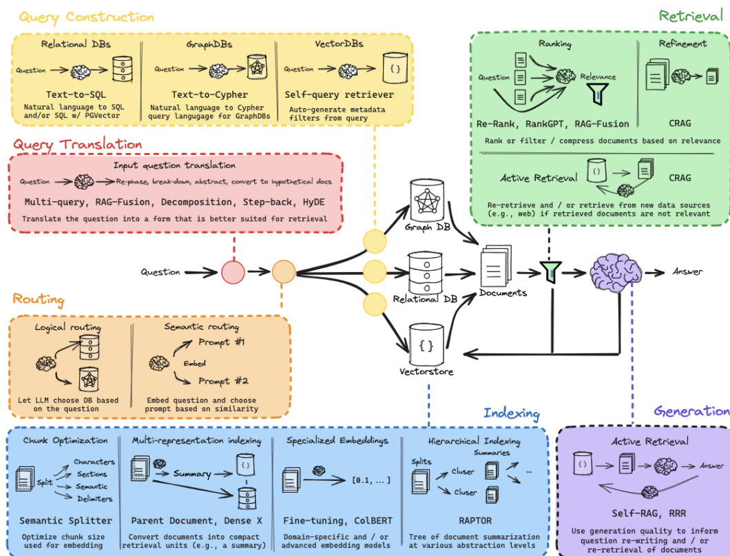
Figure 5.2: Detailed Architecture of a RAG-enhanced LLM system (source: LangChain AI [19])
