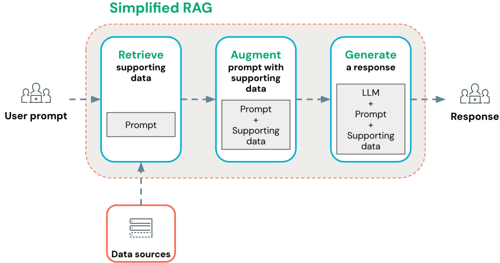
Figure 5.1: Simplified Architecture of a RAG-enhanced LLM system (source: [43])
