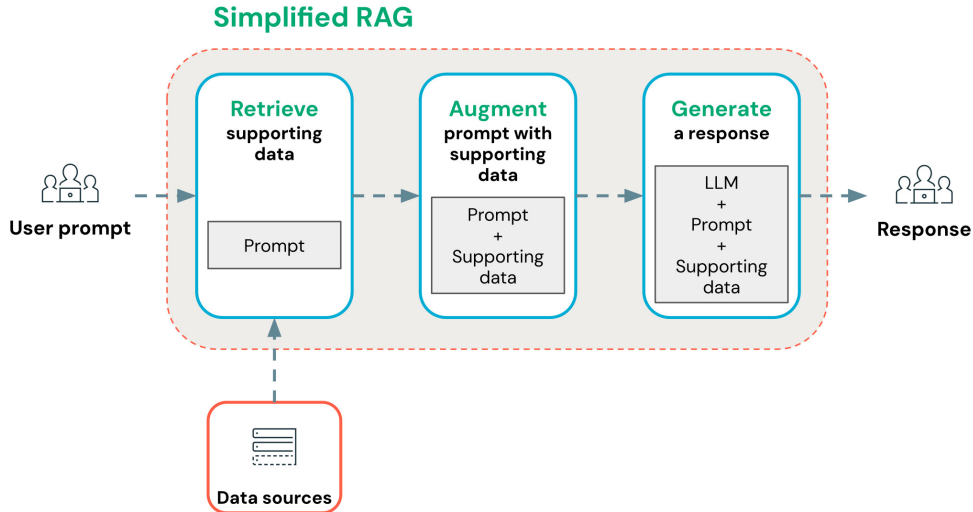
Figure 5.1: Simplified Architecture of a RAG-enhanced LLM system (source: [0])
