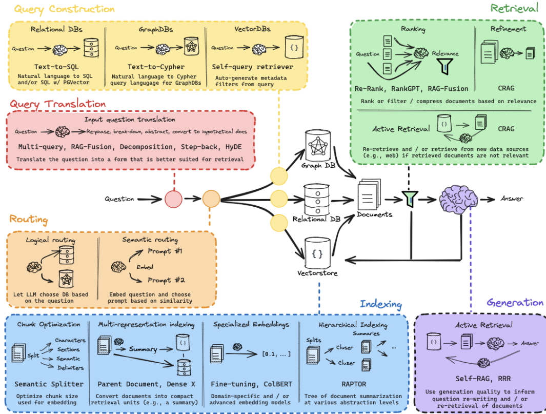
Figure 5.2: Detailed Architecture of a RAG-enhanced LLM system (source: LangChain AI [0])
