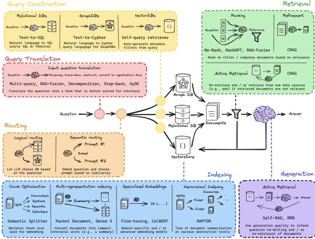
Figure 5.2: Detailed Architecture of a RAG-enhanced LLM system (source: LangChain AI [21])
