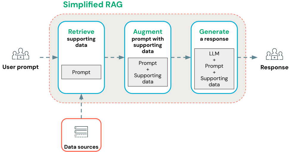
Figure 5.1: Simplified Architecture of a RAG-enhanced LLM system (source: [50])
