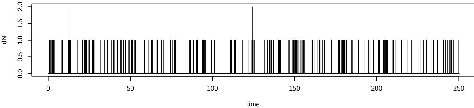
Observed events
