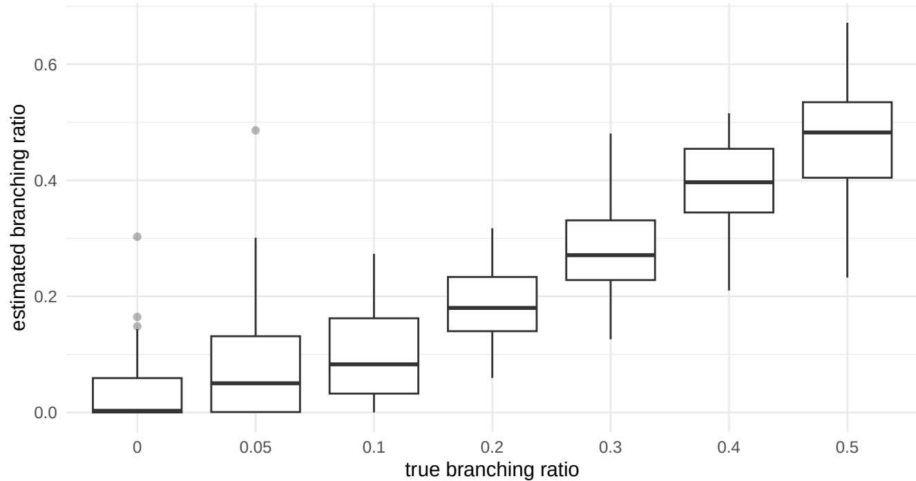
Estimated branching ratio versus true branching
