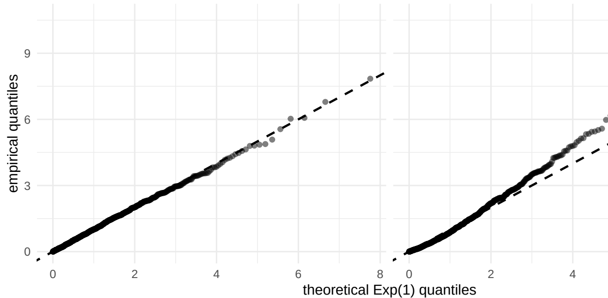
Hawkes_correct
