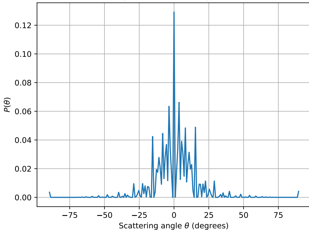
Single-slit diffraction pattern
