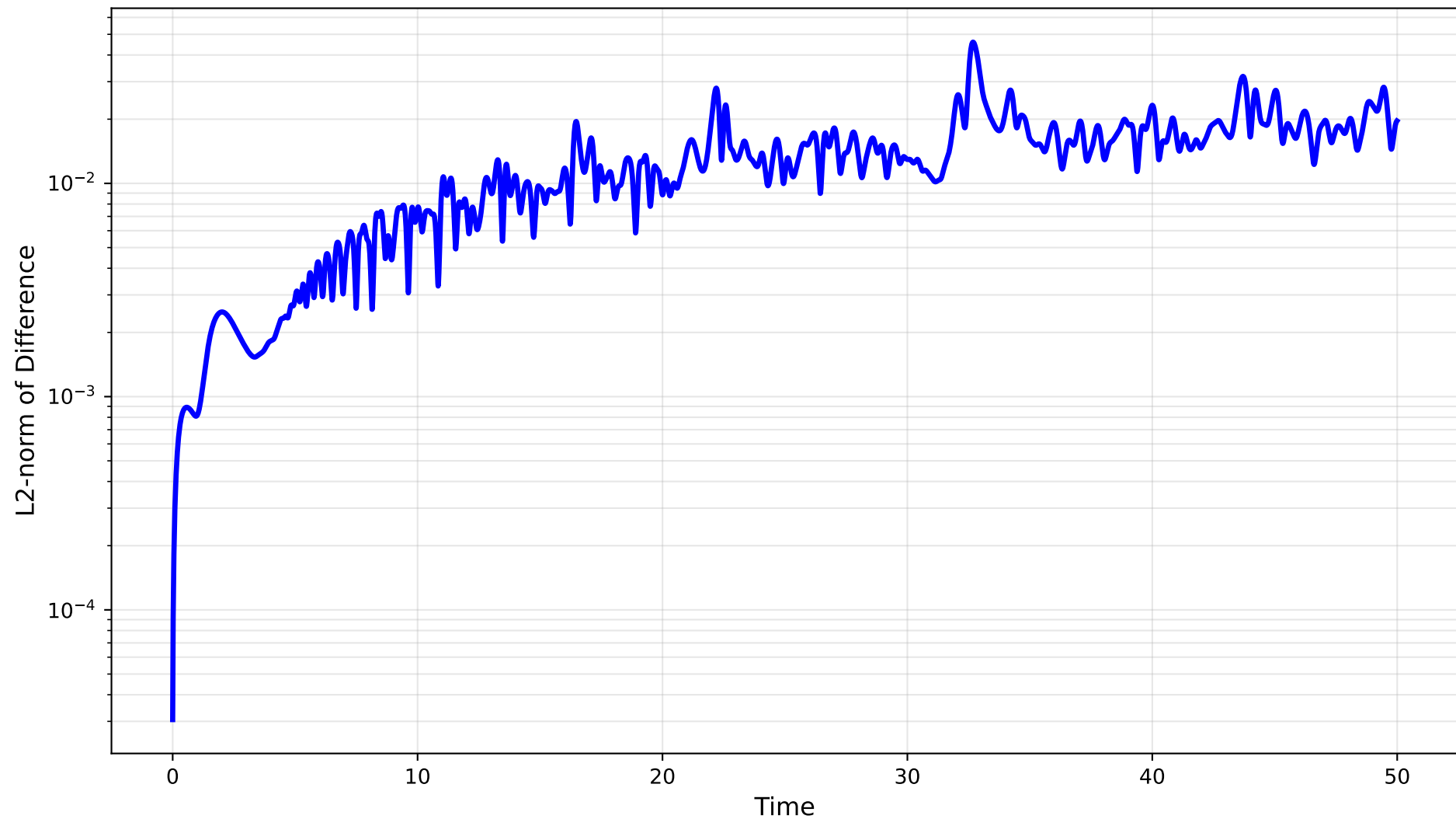
Error Growth: 5-Point vs 9-Point Stencil
