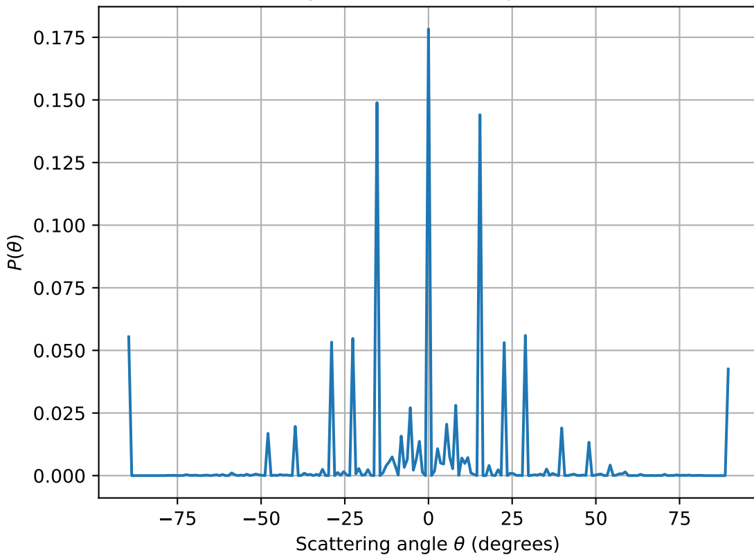
Single-slit diffraction pattern
