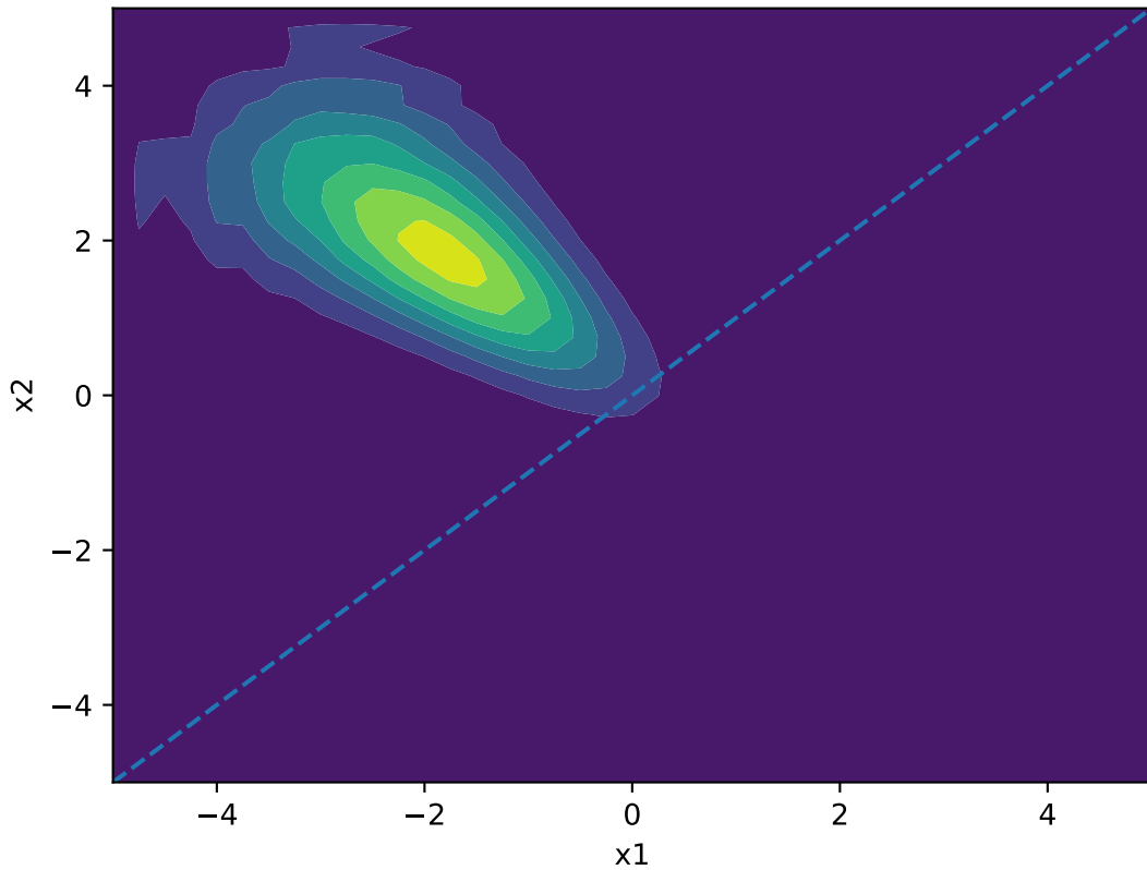
2-particle Schrodinger equation probability density
