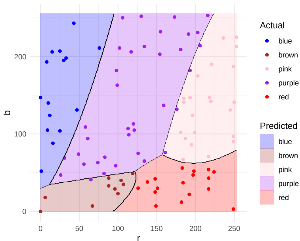
The QDA Decision Boundaries of the Classification Model
