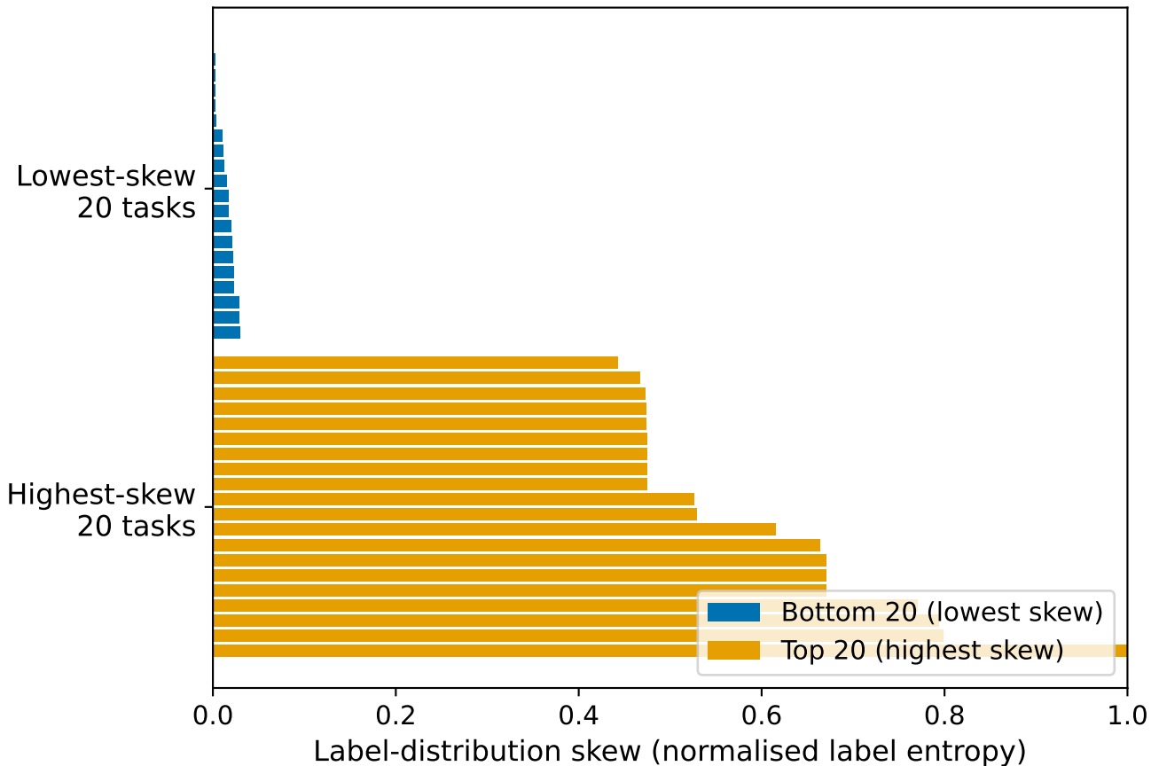
Top & bottom 20 tasks by label-distribution skew
