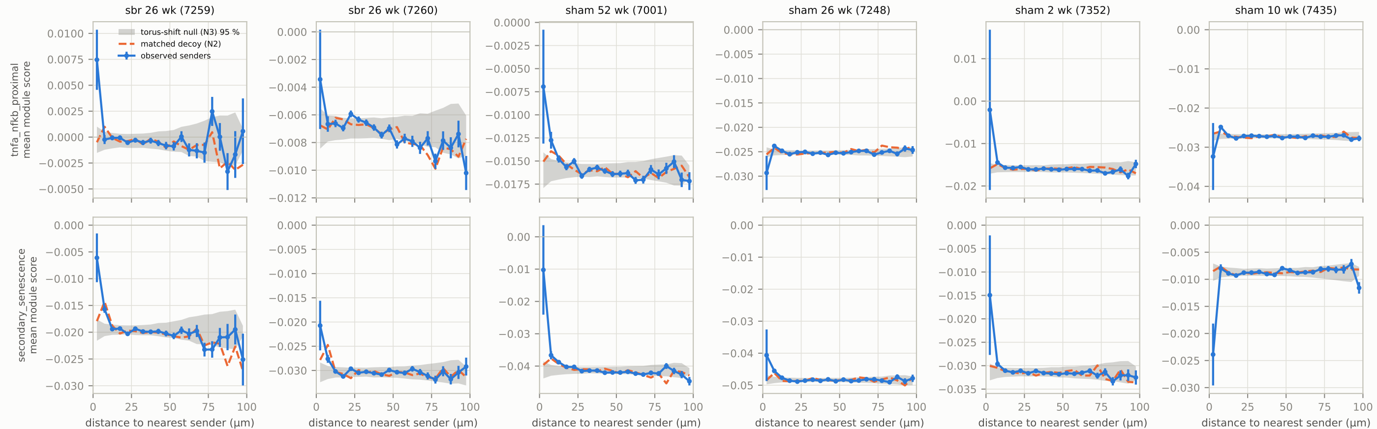
Figure 2b — the naive gradient, the matched-decoy curve and the torus-shift null band Hepatocytes, six Test-3-admissible sections, sender call tierA_p95, 5 \mu\text{m} bins to 100 \mu\text{m}
