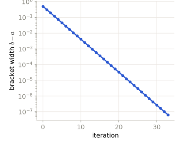
Bracket width (33 steps, \times 0.618 each)
