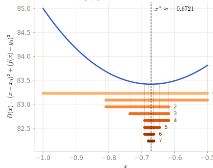
Bracket [a, b] for the first 8 iterations
