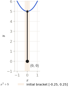
Search interval on the curve
