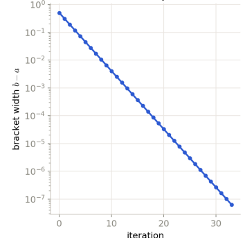
Bracket width (33 steps, \times 0.618 each)
