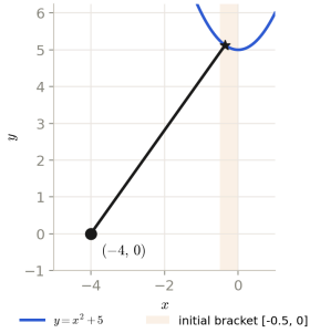
Search interval on the curve
