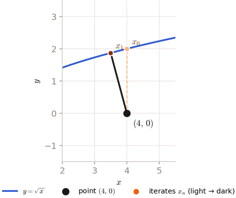
Iterates on the curve (2 steps)
