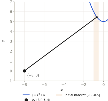
Search interval on the curve
