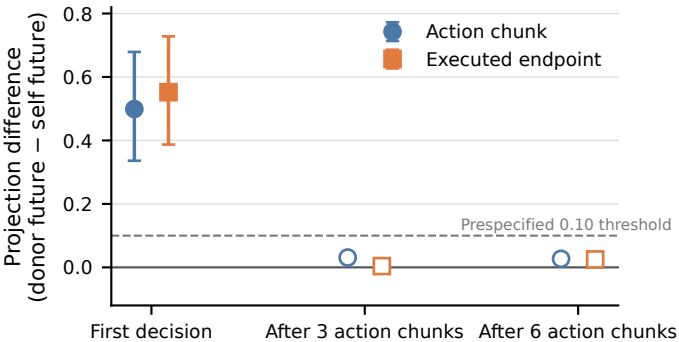
a Steering is strongest at the first query
