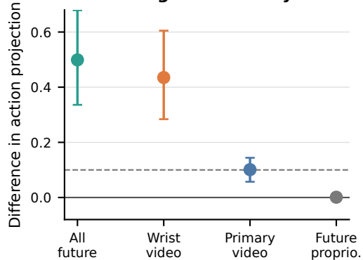
b Steering is carried by visual futures
