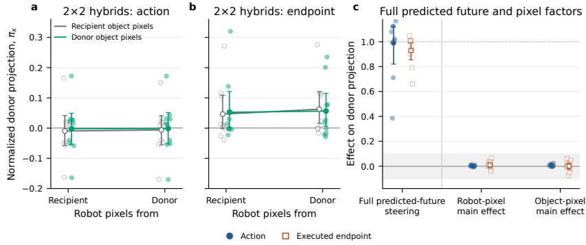
Figure 4: Cosmos 3 robot/object pixel factorization. Panels (a)–(b) show the four hybrid-video cells; panel (c) compares robot/object main effects with the full-predicted-future benchmark. Small markers are states; large markers and whiskers are means and 95% bootstrap intervals.
