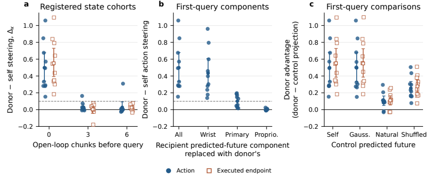
Figure 7: Cosmos Policy scope checks: (a) state cohorts, (b) predicted-future components, and (c) donor-minus-control contrasts. Small markers are tasks; large markers and whiskers are means and 95% task-bootstrap intervals.
