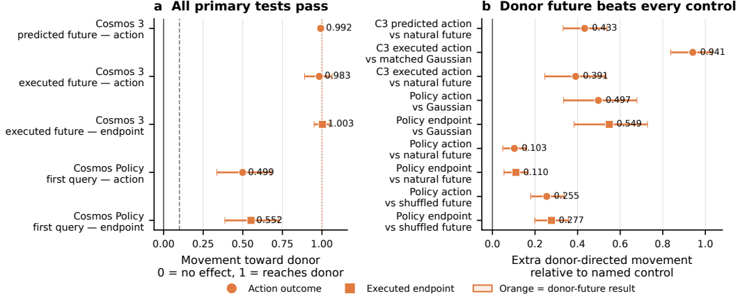
Figure 2: Does the method work? Orange always denotes a donor-future result; circles denote actions and squares denote executed endpoints. (a) All five primary donor-minus-self effects point toward the donor and their 95% bootstrap CIs exceed the prespecified 0.10 criterion. The dotted orange line marks the donor location at 1. (b) Every donor-minus-control contrast is positive: the paired donor steers more than Gaussian, natural, and shuffled alternatives. Values are printed beside each estimate.
