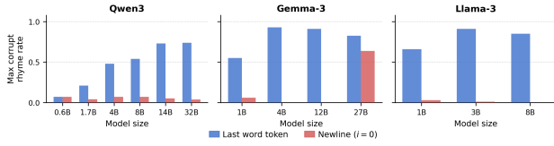
Figure 11. Peak corrupt rhyme rate (maximum across all layers) for the last word token and newline ( i = 0 ) at each model size. Gemma-3-27B is the only model for which newline patching reaches a substantial level; all Qwen3 and Llama-3 models show near-zero newline effectiveness regardless of scale.
