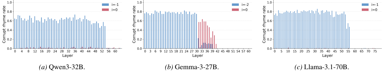
Figure 6. Per-layer activation patching at the last word token and newline ( i = 0 ) for the largest model in each family. Full results for all model sizes are in Appendix C.
