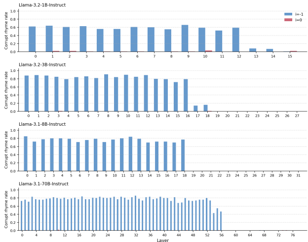
Figure 15. Per-layer activation patching, Llama-3 1B-70B.
