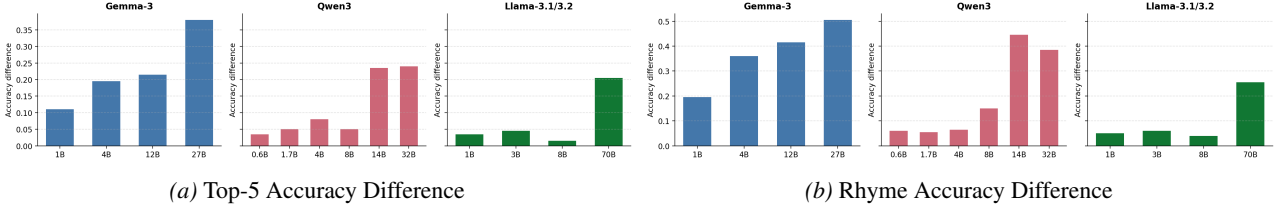
Figure 4. Maximum accuracy gap across layers between probes at the newline ( i = 0 ) and the first generated position ( i = 1 ), plotted against model size. The gap increases with scale across all three model families, suggesting that planning-compatible representations at the newline are an emergent property of larger models.
