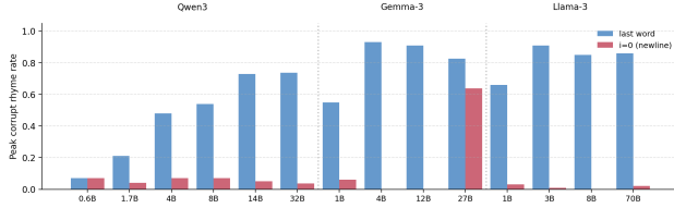
Figure 11. Peak corrupt rhyme rate (maximum across all layers) for the last word token and newline ( i = 0 ) at each model size. Gemma-3-27B is the only model for which newline patching reaches a substantial level; all Qwen3 and Llama-3 models show near-zero newline effectiveness regardless of scale.
