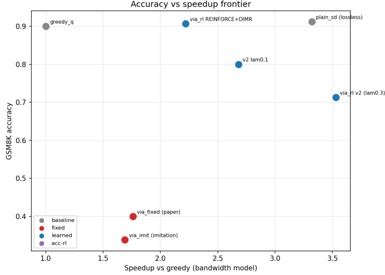
Figure 2: Accuracy vs. speedup. Learned gates dominate fixed ones; REINFORCE+DIMR matches plain SD’s accuracy (0.907) at lower speed (the q' overhead); v2 trades accuracy for speed.
