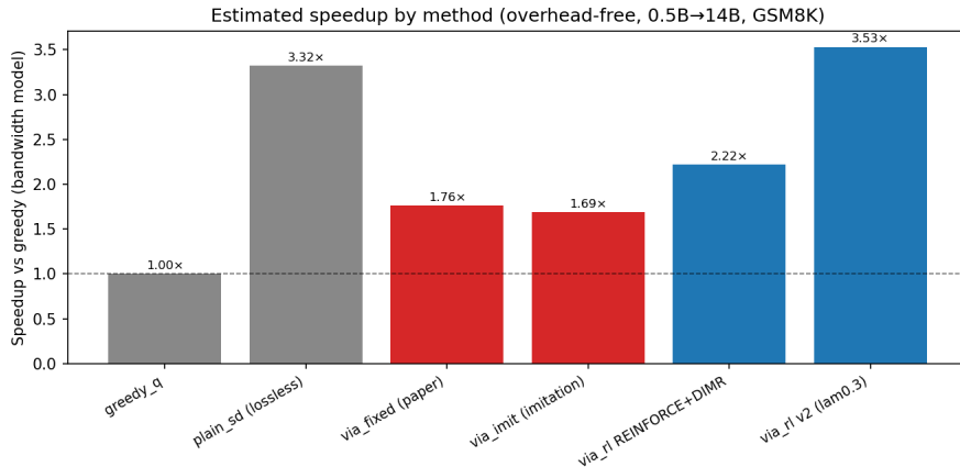
Figure 1: Overhead-free speedup by method. The learned v2 gate and plain SD reach \sim 3.3\text{--}3.5\times ; the fixed-threshold gate is slow because it over-escalates to the full model.
