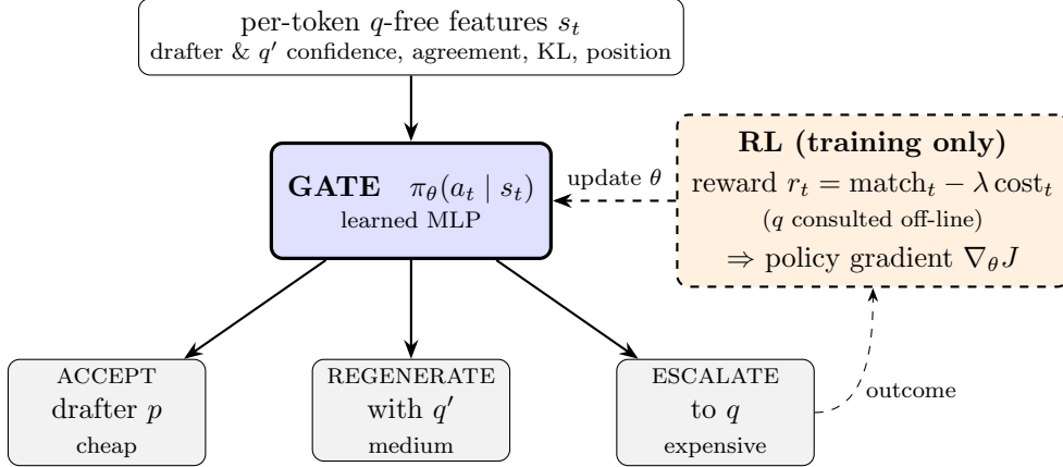
Figure 1: Method overview. The learned gate is the central component. For each drafted token it reads the q -free features s_t and routes the token to one of three tiers: accept (drafter), regenerate (slim q' ), or escalate (full q ). Reinforcement learning enters only at training time, shown by the dashed path. Each action’s outcome yields a reward r_t = \text{match}_t - \lambda \text{cost}_t , computed with q off-line, and a policy-gradient step updates the gate parameters \theta . At inference the dashed path is removed, and the gate runs from the q -free features alone.
