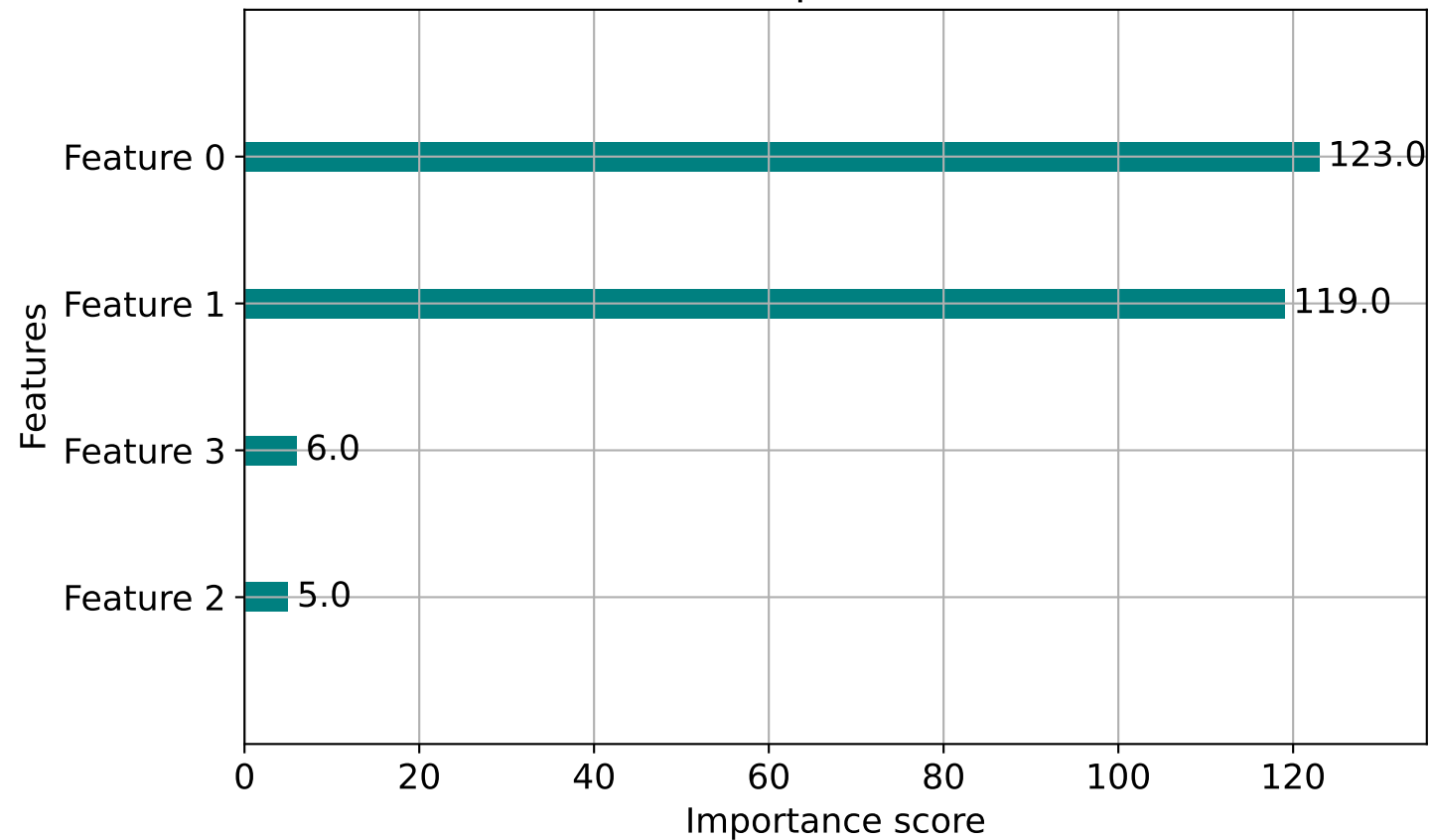
XGBOOST Feature Importance (10-tree model)
