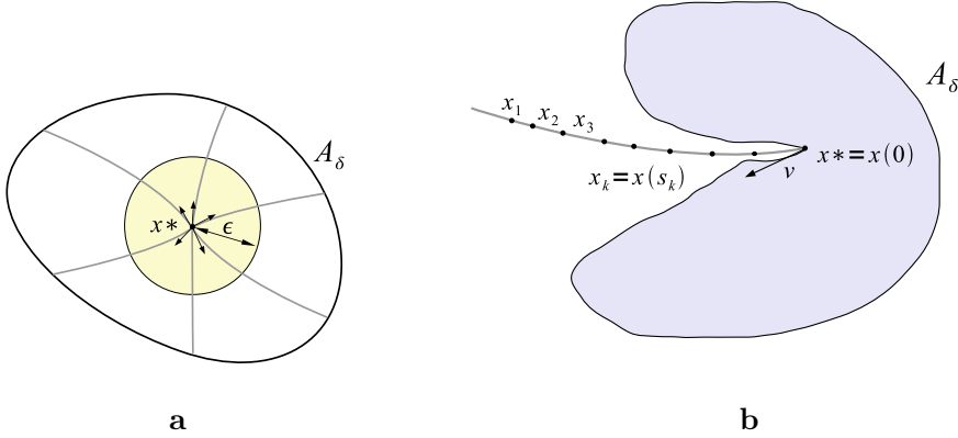
Figure 4.4: a. There is a ball B(x^*, \epsilon) included in A_\delta . b. The sequence (x_k)_k tends to x^* along the curve x(s) .
