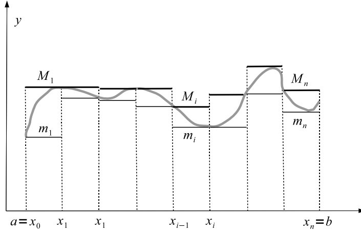
Figure 15.1: When n increases, the difference M_i - m_i decreases towards zero.
