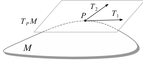
Figure 13.3: The tangent space T_p \mathcal{M} .
