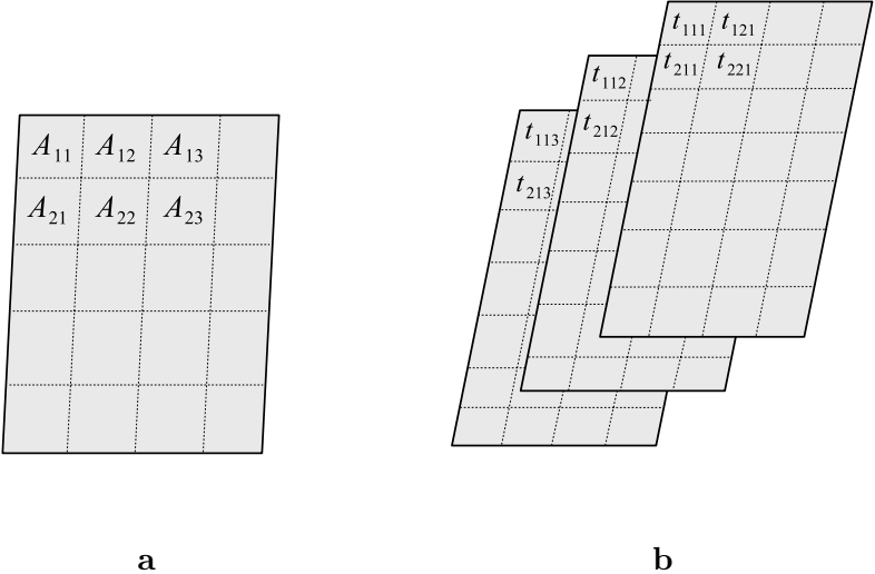
Figure 1: a. An order 2 tensor A \in \mathbb{R}^{5 \times 4} . b. An order 3 tensor t \in \mathbb{R}^{7 \times 4 \times 3} .
