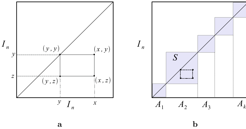
Figure 18.2: a. The rectangle rule: if (x, y), (y, y), (y, z) \in \mathcal{S} , then (x, z) \in \mathcal{S} . b. Equivalence relation \mathcal{S} , which makes a finite partition of I_n .
