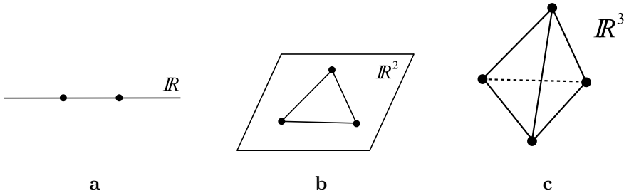
Figure 18.5: Points in a general position: a. Two distinct points on a line. b. Three noncollinear points in the plane. c. Four noncoplanar points in 3-dimensional space.
