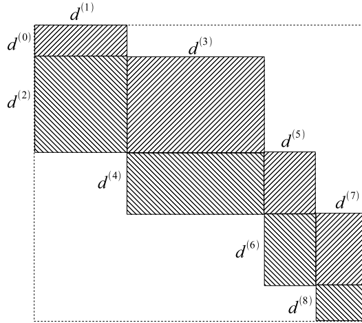
Figure 13.8: The area significance of the sum d^{(0)}d^{(1)} + d^{(1)}d^{(2)} + \dots + d^{(7)}d^{(8)} .
