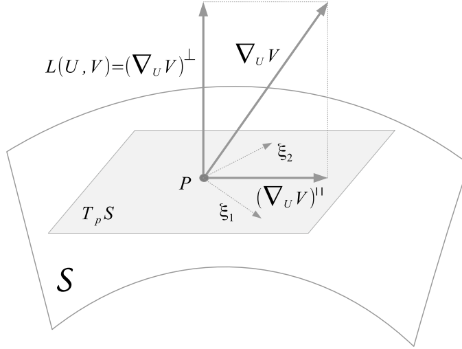
Figure 13.4: Gauss formula \nabla_U V = (\nabla_U V)^{\parallel} + L(U, V) .
