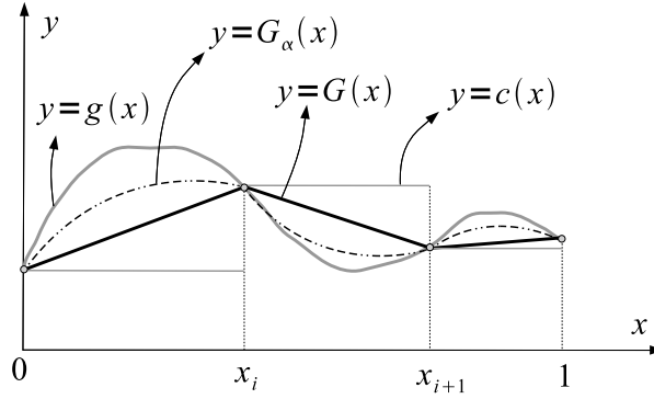
Figure 8.10: The approximation of a continuous function g \in C[0, 1] by three approximators: G(x) = \sum_{j=0}^{N-1} \alpha_j \text{ReLU}(x - x_j) + \beta , G_\alpha(x) = \sum_{j=0}^{N-1} c_j \text{sp}(wx - \theta_j) + \beta and c(x) = \sum_{i=0}^{N-1} c_i H(x - x_i) .
