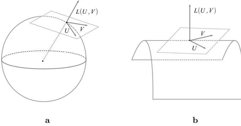
Figure 13.5: The second fundamental form is normal to the surface and describes its shape: a. The case of a sphere. b. The case of a cylindrical surface.
