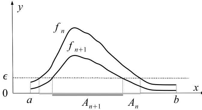
Figure 7.1: The descending sequence of compact sets A_n .
