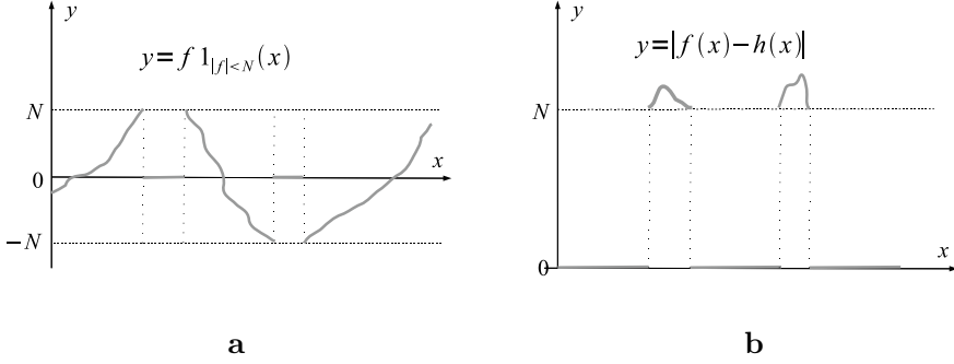
Figure 9.5: a. The graph of y = h(x) . b. The graph of y = |f(x) - h(x)| .
