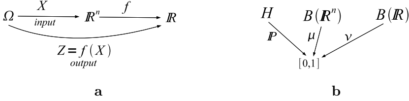
Figure 11.4: a. The input and output variables. b. The measures \mathbb{P} , \mu , and \nu .
