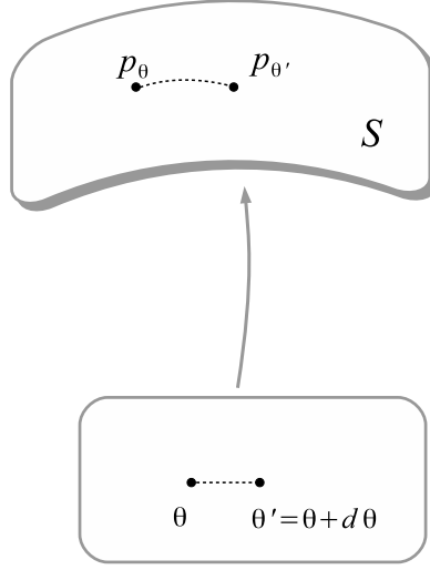
Figure 14.5: The Riemannian distance between \theta and \theta' is related to the Kullback-Leibler divergence of p_\theta and p_{\theta'} .
