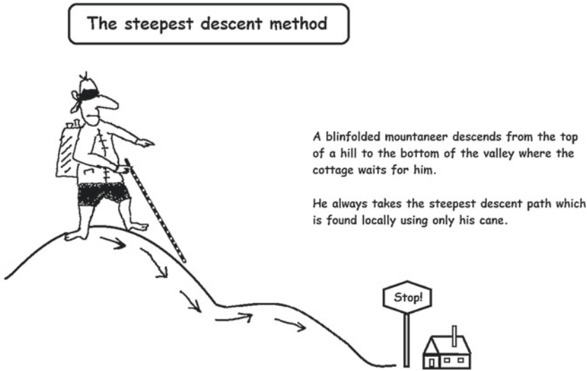
Cartoon 1: A blindfolded man gets off a mountain using the steepest descent method by taking advantage of the local geometry of the environment.
