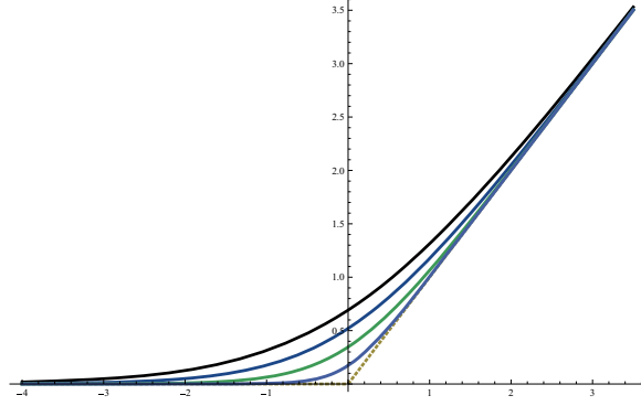
Figure 8.9: The scaled softplus \varphi_\alpha(x) for values \alpha = 1, 0.75, 0.5, 0.25 .
