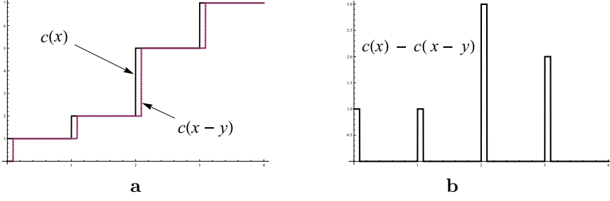
Figure 8.5: a. The step functions c(x) and c(x - y) for |y| < \epsilon' . b. The graph of the difference c(x) - c(x - y) .
