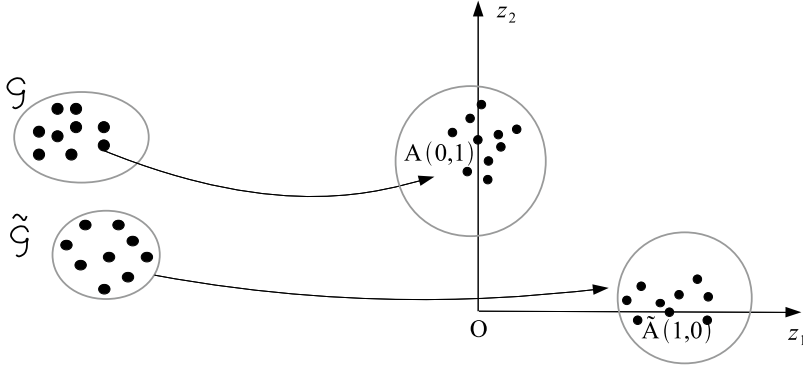
Figure 18.13: The linearly separable clusters \mathcal{G} , \tilde{\mathcal{G}} are mapped into disjoint neighborhoods of point labels A and \tilde{A} .
