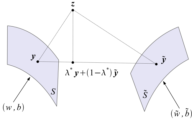
Figure 13.17: The orthogonal projection of \mathbf{z} on the line segment \mathbf{y}\tilde{\mathbf{y}} is a better approximator than both \mathbf{y} and \tilde{\mathbf{y}} . This is given by \lambda^* \mathbf{y} + (1 - \lambda^*) \tilde{\mathbf{y}} , where \lambda^* is obtained as \lambda^* = \arg \min \|\mathbf{z} - \lambda \mathbf{y} - (1 - \lambda) \tilde{\mathbf{y}}\| .
