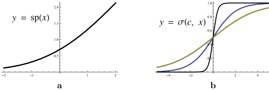
Figure 2.7: a. Softplus function sp(x) = \ln(1 + e^x) b. Family of logistic functions approximating the step function.
