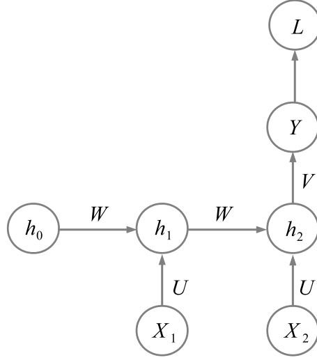
Figure 5: A “2-to-1” RNN for Exercise 17.10.3.
