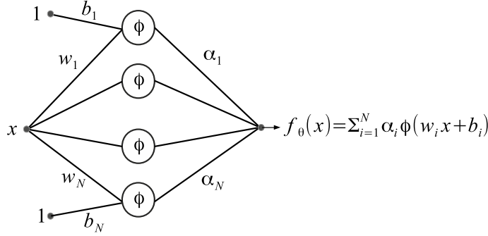
Figure 14.3: One-hidden layer neural network with activation function \phi and input-output mapping f_\theta(x) . The activation in the output neuron is linear.
