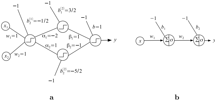
Figure 6.7: a. Neural network used in Exercise 6.6.3. b. For Exercise 6.6.6.
