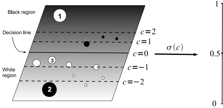
Figure 5.9: The family of lines w_1x_1 + w_2x_2 - b = c , c \in \mathbb{R} . The sigmoid function \sigma maps each line to a point in (0, 1) regarded as a probability.
