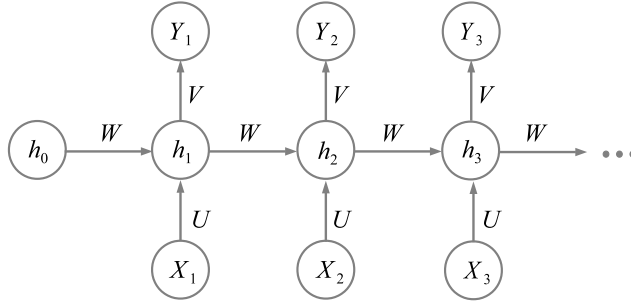
Figure 17.2: A “many-to-many” configuration of an RNN.
