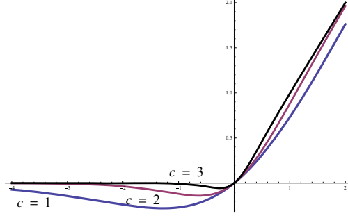
Figure 2.6: The activation function \phi_c(x) = x\sigma(cx) = \frac{x}{1+e^{-cx}} for c = 1, 2, 3 .
