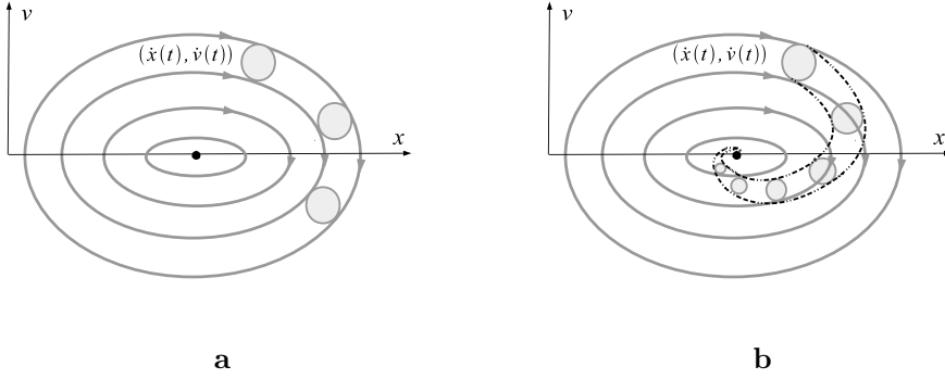
Figure 4.12: Solution in phase space: a. The divergence of the tangent flow is zero and the volumes are preserved along the flow. The solution oscillates forever around the equilibrium point. b. When friction forces are present the tangent flow shrinks and the trajectory evolves to lower levels of energy. The oscillation is amortized in time.
