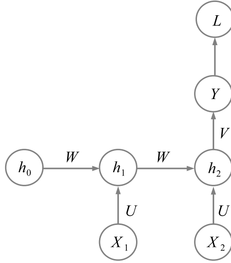
Figure 17.5: A “2-to-1” RNN for Exercise 17.10.3.
