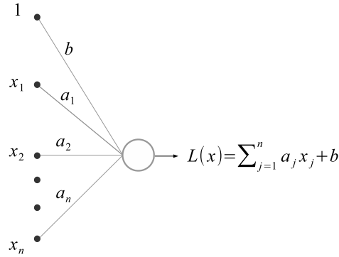
Figure 1.7: A linear approximator neuron .
