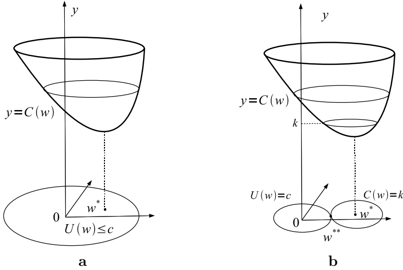
Figure 3.4: The cost function C(w, b) in two distinguished possibilities: a. w^* \in \{w; U(w) \leq c\} b. w^* \notin \{w; U(w) \leq c\} .
