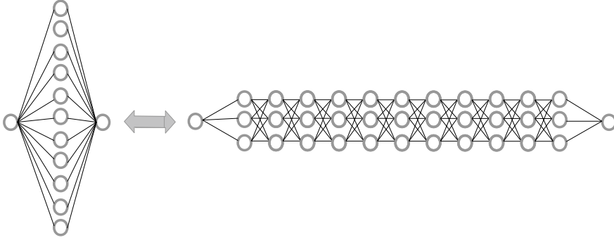
Figure 10.4: Two ReLU-networks, one “shallow and wide” and the other, “deep and narrow” can compute the same function.
