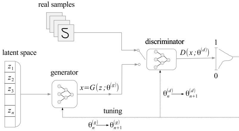
Figure 19.2: The anatomy of a GAN: latent variables are fed into the generator producing “fake” data. Then repeatedly sample two minibatches of data, one from the real data and another from the generated data and let the discriminator decide whether it is fake or genuine. Using this decision, we can update the networks parameters to improve the GANs functionality.
