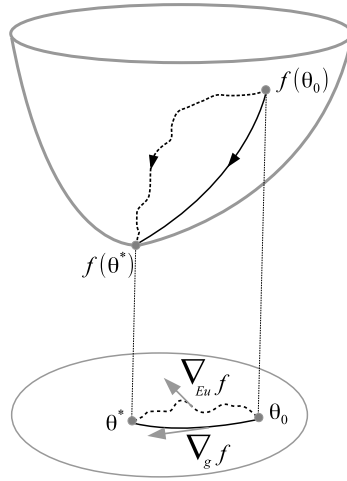
Figure 14.4: The natural gradient descent arrives faster to the minimum than the Euclidean gradient descent method does.
