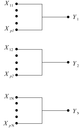
Figure 15.3: Max-pooling layer with Y_j = \max\{X_{1j}, \dots, X_{pj}\} , 1 \leq j \leq N .
