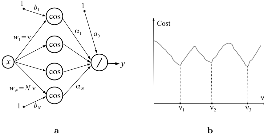
Figure 7.3: a. One-hidden neural network with cosine activation functions. b. The cost function reaches its relative minima for certain values of the hyperparameter \nu .
