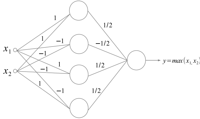
Figure 10.1: A one-hidden layer network learning exactly the maximum of two numbers.
