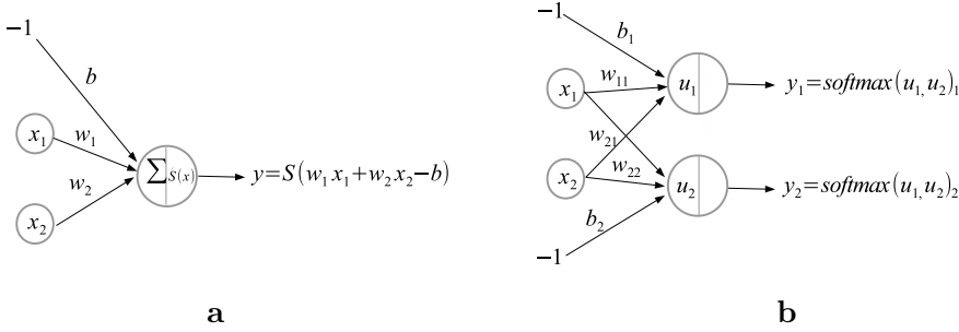
Figure 5.8: a. The neuron in the case when the labels are z \in \{-1, 1\} . b. The neural networks in the case of one-hot-vector labels.
