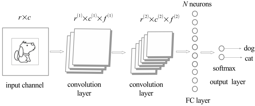
Figure 16.7: CNN with two convolution layers, one fully-connected layer and a softmax layer (output layer).
