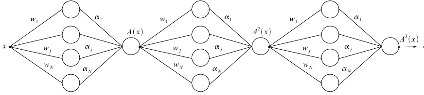
Figure 7.5: A recurrent neural net constructed from three-layer neural units.
