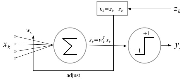
Figure 5.12: Adaline neuron .
