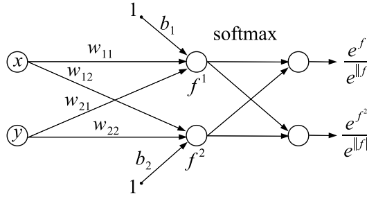
Figure 18.14: Neural network with an extra layer implementing the softmax function.
