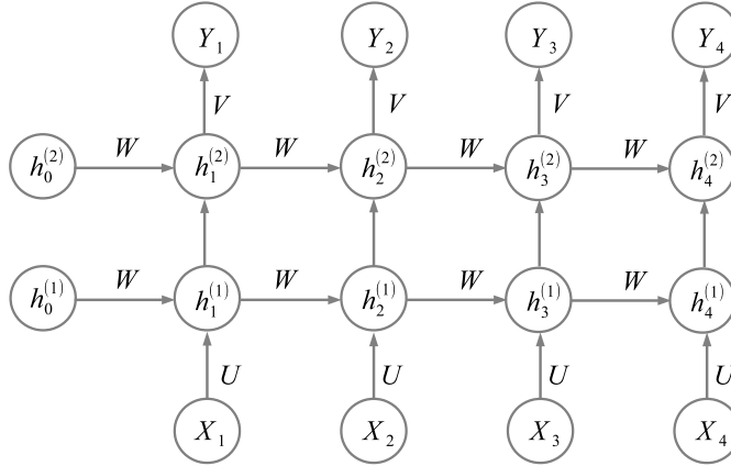
Figure 17.4: A deep RNN with T = 4 and L = 2 .
