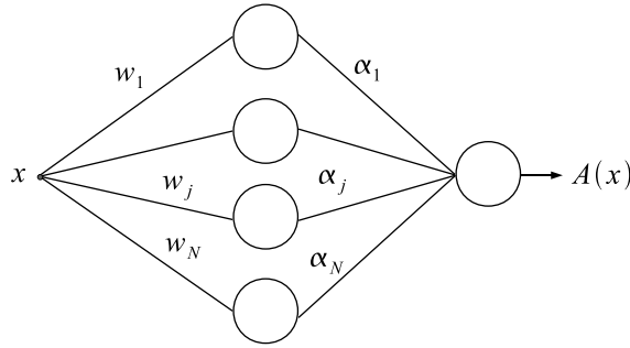
Figure 7.4: A three-layer neural unit whose output is a contraction.
