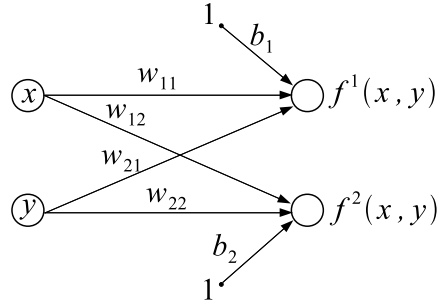
Figure 18.12: Neural network with no hidden layers and two outputs.
