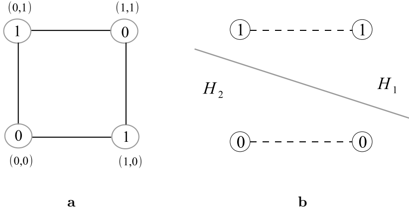
Figure 5.6: Cluster classification using one perceptron: a. The output function XOR. b. A line divides the plane in two convex sets H_1 and H_2 .
