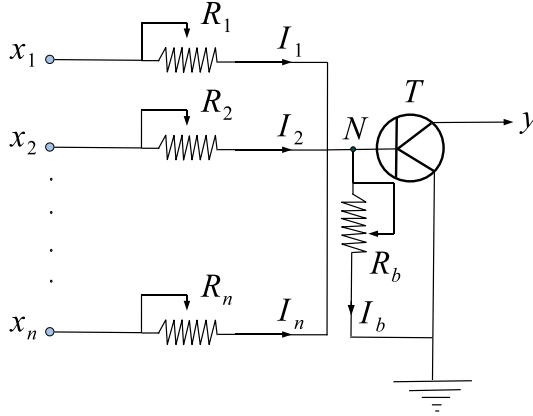
Figure 1.2: The neuron implemented as an electronic circuit.
