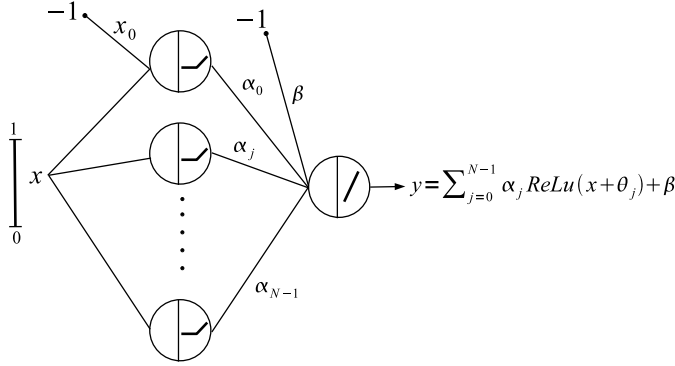
Figure 8.7: One-hidden layer neural network with ReLU activation functions.
