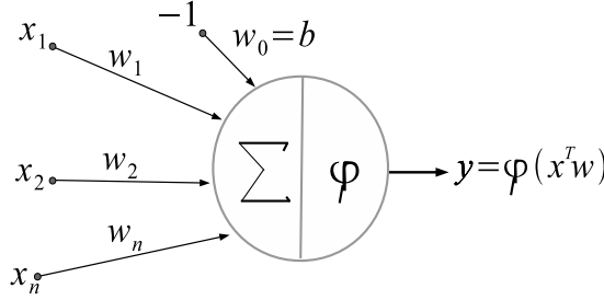
Figure 5.1: Abstract neuron with bias b and activation function \varphi .
