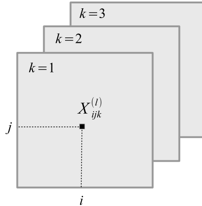
Figure 16.6: The entries of the tensor X^{(\ell)} \in \mathbb{R}^{r^{(\ell)} \times c^{(\ell)} \times 3} . The entry X_{ijk}^{(\ell)} represents the activation in the spatial location (i, j) situated in the k th channel.
