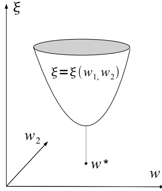
Figure 5.11: The quadratic error function has a global minimum \mathbf{w}^* .
