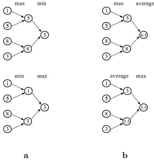
Figure 3: For Exercise 15.6.5: a. Switching a min-pooling with a max-pooling layer provides different outputs. b. Switching an average-pooling with a max-pooling layer provides different outputs.
