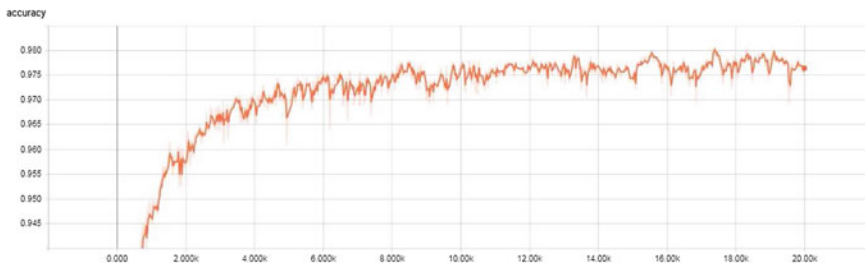
Figure 12.11: A one-hidden layer feedforward network, with 300 neurons in the hidden layer, trained with a batch size of 40, using the ReLU and the softmax activation functions for the hidden and output layer, respectively, produces a testing accuracy of 97.6%. The learning uses ADAM method with learning rate starting at \lambda = 0.0015 . The cost function used is the cross-entropy. The diagram was generated with Tensorboard.
