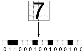
Figure 5.2: Transformation of a 4 \times 4 pixels character into a sequence of 0s and 1s.
