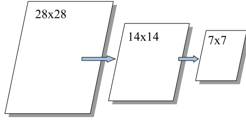
Figure 15.4: Two max-pooling layers applied to an MNIST image.
