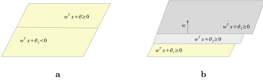
Figure 11.7: a. Information generated by a perceptron. b. Information generated by a sigmoid or a linear neuron.
