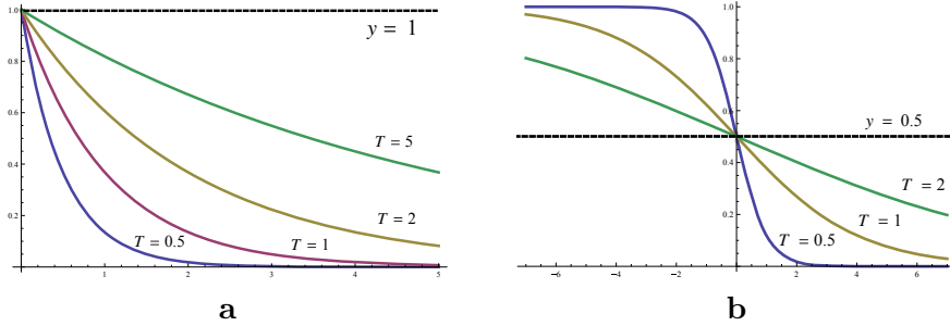
Figure 4.16: a. The Boltzmann distribution p(x) = e^{-x/T} . b. The reflected sigmoid functions f(x) = \frac{1}{1+e^{x/T}} . Both functions are represented for a few different values of T .
