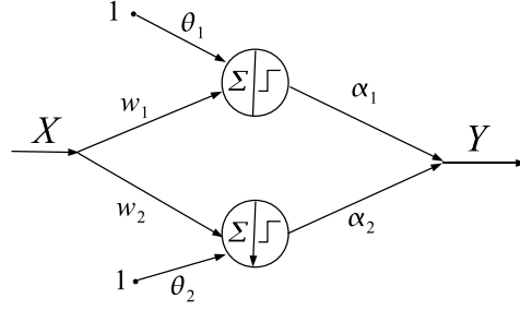
Figure 11.8: Neural networks made of two perceptrons. Its output is given by Y = \alpha_1 H(w_1^T X + \theta_1) + \alpha_2 H(w_2^T X + \theta_2) .
