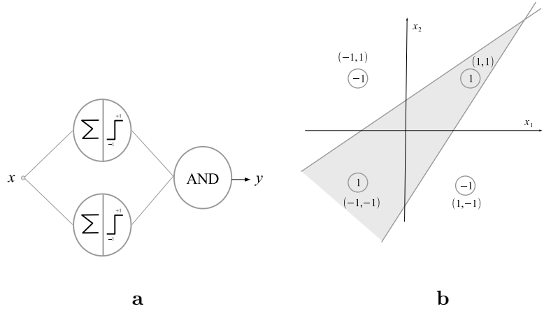
Figure 5.13: a. Madaline with two Adaline units. b. Madaline implementation of XNOR function. The Madaline takes value 1 on the shaded area and value -1 in rest.
