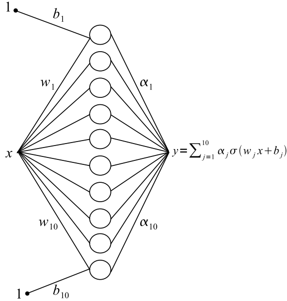
Figure 13.6: A one-hidden layer neural network with N = 10 hidden neurons, which depends on 30 parameters.
