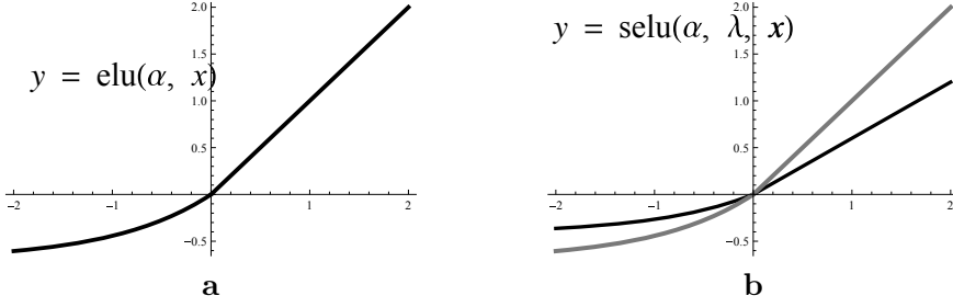
Figure 2.4: Hockey-stick functions: a. y(x) = ELU(\alpha, x) b. y(x) = SELU(\alpha, \lambda, x) .
