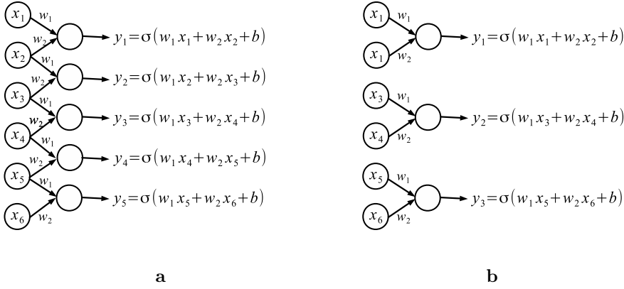
Figure 16.2: Two convolution layers: a stride equal to 1; b stride equal to 2. All missing arrows are assigned a zero weight. All neurons have the same bias b .
