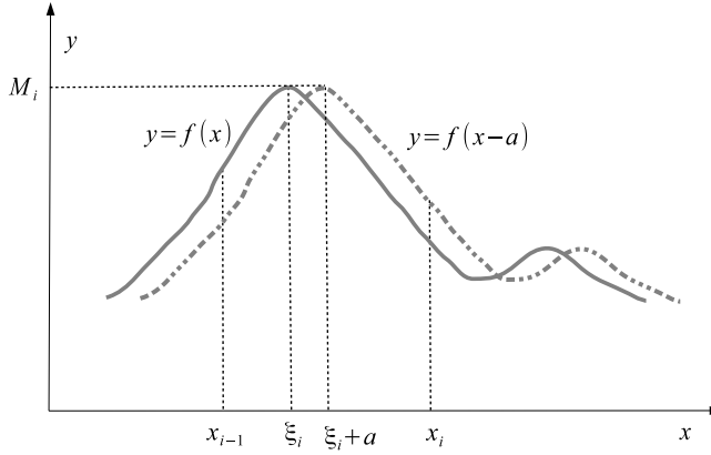
Figure 15.2: Max-pooling for f and T_a \circ f .
