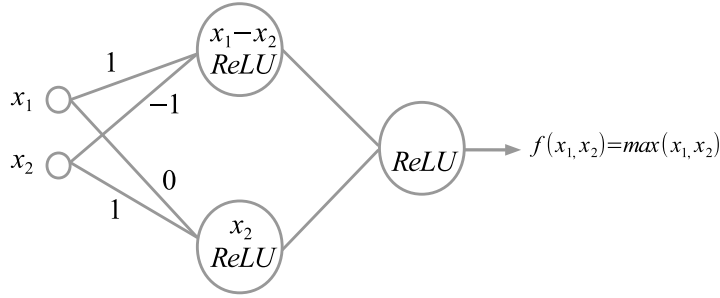
Figure 10.3: A neural network learning exactly the maximum of 2 numbers.
