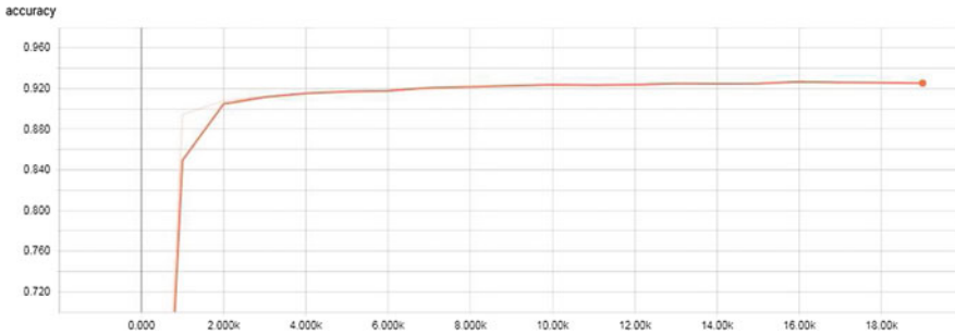
Figure 12.10: A zero-hidden layer feedforward network using a batch size of 30, the softmax activation function, and the gradient descent method with learning rate \lambda = 0.03 , producing a testing accuracy of 92.5%. The network uses a cost function given by the sum of squares. The diagram was generated with Tensorboard.
