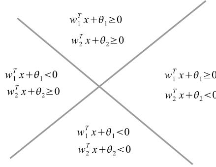
Figure 11.9: Information provided by a network of two classical perceptrons.
