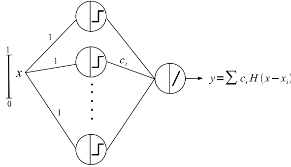
Figure 8.2: A one-hidden layer perceptron network with input to hidden layer weights equal to 1 and hidden layer to output weights equal to c_i ; the biases are given by x_i .
