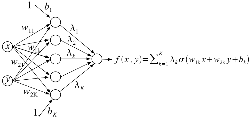
Figure 18.18: Neural network with one-hidden layer and one output.
