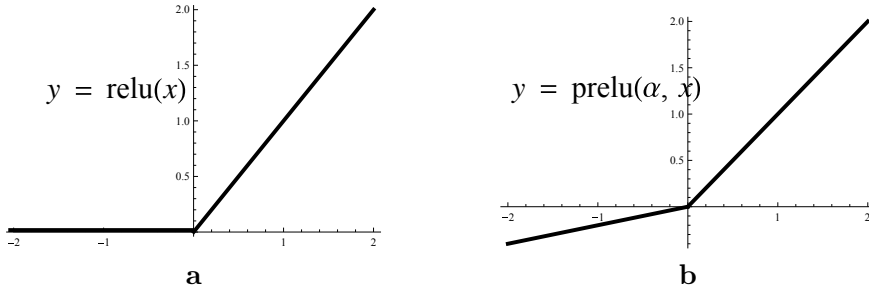
Figure 2.3: Hockey-stick functions : a. y = \text{ReLU}(x) b. y = \text{PReLU}(\alpha, x) .
