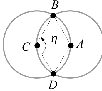
Figure 4.20: Two equal circles intersect at points B and D and also pass through the centers of each other. Triangles \triangle ABC and \triangle ACD are equilateral, having all sides equal to \eta . Therefore the angle \angle BCD = 120^\circ and hence the arc BAD represents 1/3 of the total circle circumference, which means that the circle centered at C has 2/3 outside of the other circle.
