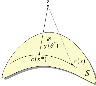
Figure 13.12: The optimum parameter, s^* , corresponds to the closest point on the curve c(s) to the target \mathbf{z} .
