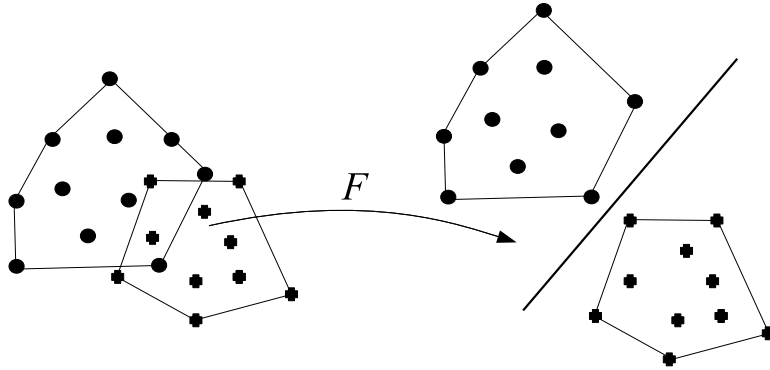
Figure 18.8: The separation function F of two intersecting clusters is nonlinear.
