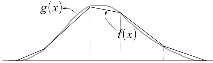
Figure 9.6: A piecewise continuous function \ell(x) approaches uniformly the compact supported continuous function g(x) .
