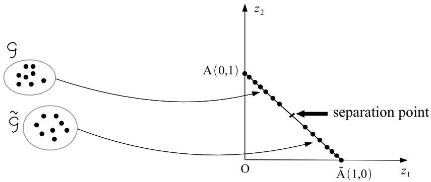
Figure 18.15: The linearly separable clusters \mathcal{G} and \tilde{\mathcal{G}} are mapped into the terminal regions of a line segment. In the interior of the segment there is a separation point.
