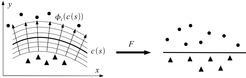
Figure 18.20: The function F maps the decision curve into the x -axis.
