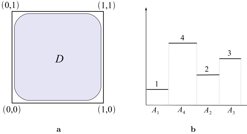
Figure 18.3: a. Subset D in I_2 with the Lebesgue measure of the complement small. b. Decision function associated with a partition.
