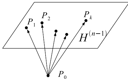
Figure 18.6: The points P_1, \dots, P_k are in a general position if the vectors \overrightarrow{P_0 P_j} are linearly independent.
