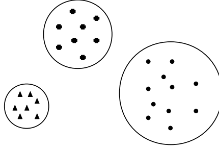
Figure 18.9: The convex separation of three clusters.
