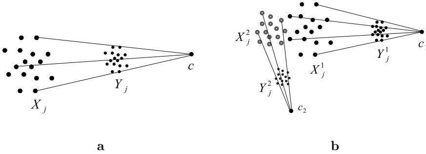
Figure 18.11: a. Contraction of a cluster toward a point. b. Contraction of two clusters toward two distinct points.
