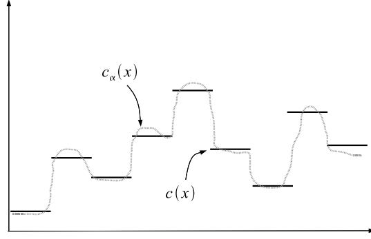
Figure 8.4: The step function c(x) and its “smoother” c_\alpha(x) = (c * \psi_\alpha)(x) .
