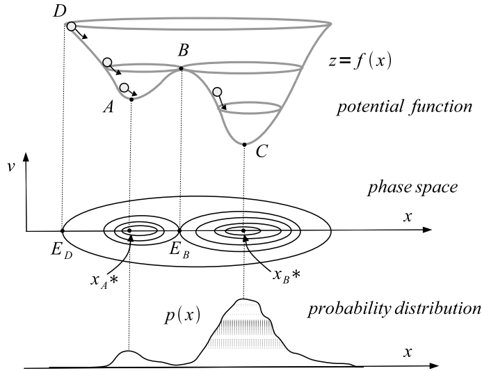
Figure 4.14: Potential function, phase space representation and final distribution of particles.
