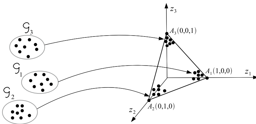
Figure 18.16: The linearly separable clusters \mathcal{G}_1 , \mathcal{G}_2 and \mathcal{G}_3 are mapped into the vertex regions of a triangle.
