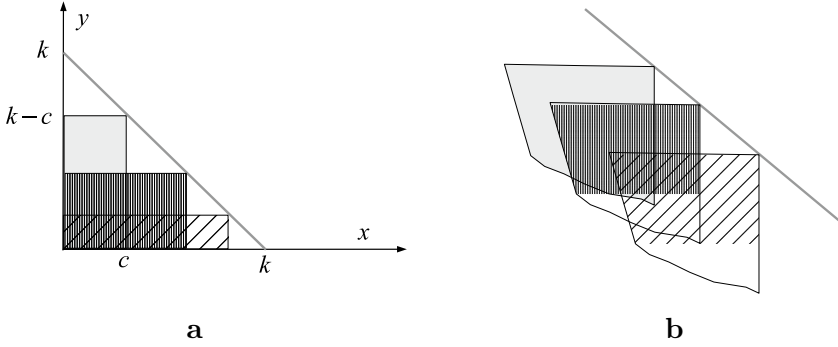
Figure 11.10: a. Triangle as a union of rectangles. b. Half-space as a union of infinite rectangles.
