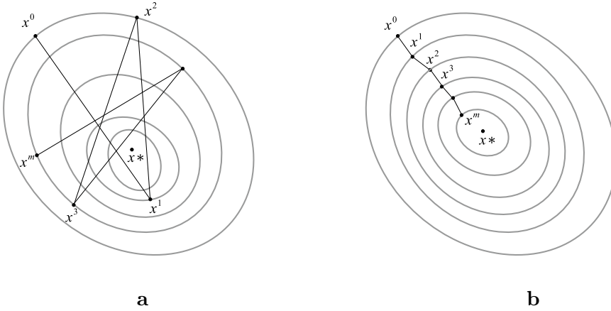
Figure 4.6: The polygonal line \mathfrak{P}_m = [x^0, \dots, x^m] in two cases: a. Step \eta large. b. Step \eta small.
