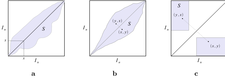
Figure 18.1: a. Reflexive, nonsymmetric relation. b. Reflexive and symmetric relation. c. Symmetric nonreflexive relation.
