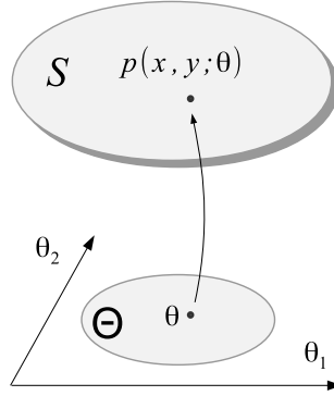
Figure 14.1: A statistical manifold \mathcal{S} = \{p(x, y; \theta); \theta \in \Theta\} .
