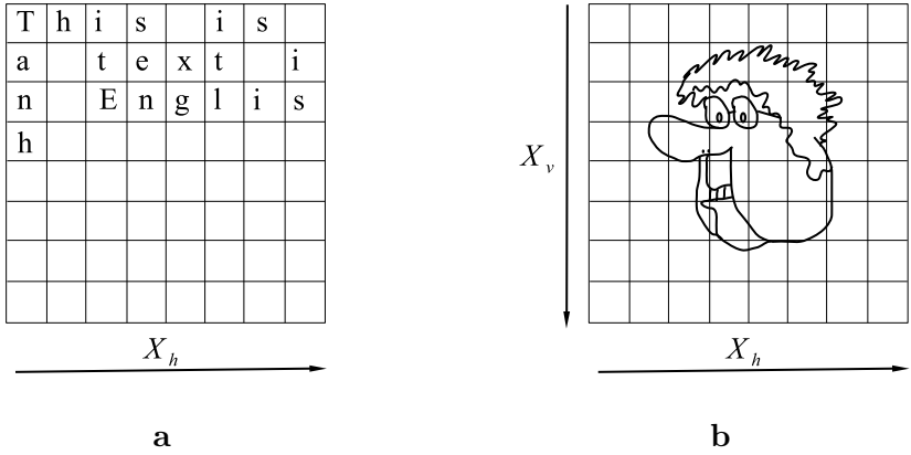
Figure 12.12: (a) The information is given only by the horizontal component: H(X_h, X_v) = H(X_h) ; (b) The information has both horizontal and vertical components: H(X_h, X_v) = H(X_h) + H(X_v) - I(X_h, X_v) .
