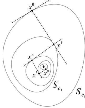
Figure 4.10: The approximation of the minimum x^* by the method of line search.
