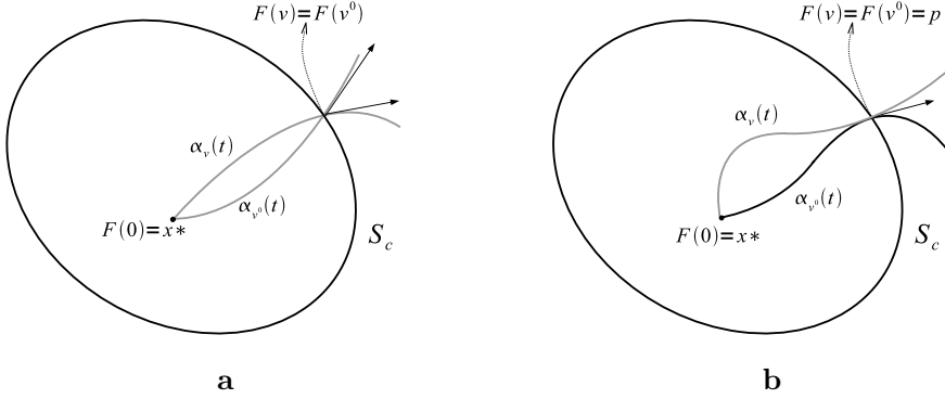
Figure 4.5: The existence of a cut-point: a. The curves \alpha_v and \alpha_{v^0} are transversal. b. The curves \alpha_v and \alpha_{v^0} are tangent.
