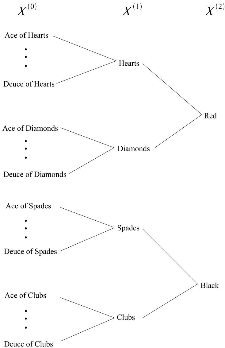
Figure 12.4: The Markov chain X^{(0)} \rightarrow X^{(1)} \rightarrow X^{(2)} , where X^{(0)} is the identity of a card, X^{(1)} is the suit of a card, and X^{(2)} is the color of a card.
