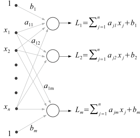
Figure 1.8: A linear approximator neural net.
