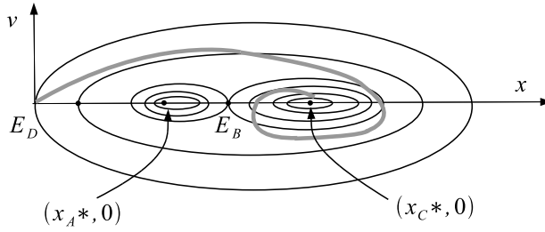
Figure 4.15: Most of damped trajectories will spiral in approaching the equilibrium point (x_C^*, 0) , which has a larger basin of attraction.
