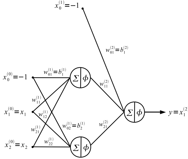
Figure 6.2: Neural network with one hidden layer, having two inputs, x_1, x_2 , and two neurons in the hidden layer.
