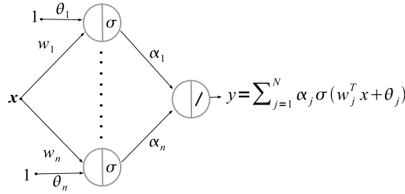
Figure 9.2: The one-hidden layer neural network which approximates continuous functions.
