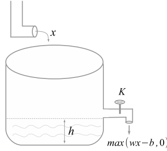
Figure 1.9: A water tank with a knob and outflow \phi(x) = \max(wx - b, 0) .
