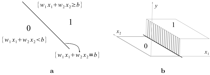
Figure 5.3: a. The separation of the plane into half-planes. b. The graph of the activation function for a perceptron with two inputs, x_1 and x_2 .
