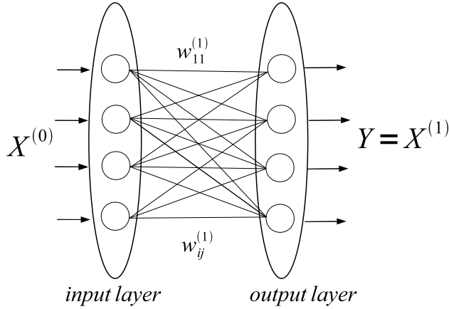
Figure 11.12: A two-layer neural network with d^{(0)} = d^{(1)} .
