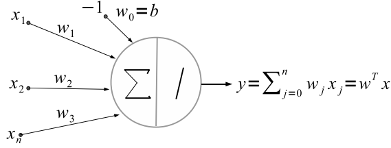
Figure 5.10: Linear neuron with bias b and linear activation function.
