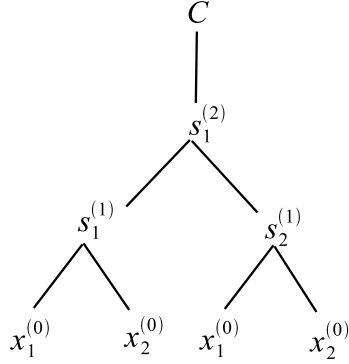
Figure 6.4: The dependence tree used for applying chain rule.
