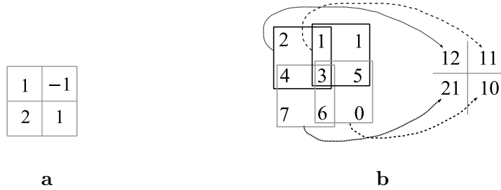
Figure 16.5: The convolution operation: a A 2 \times 2 kernel; b the input and output of a convolution.
