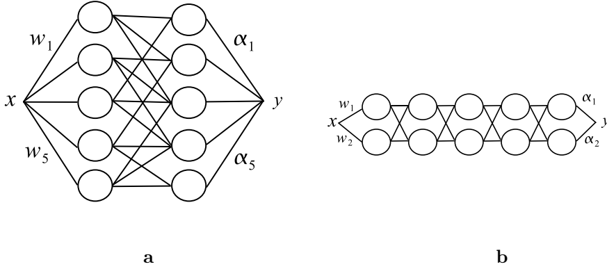
Figure 13.7: Two neural nets with N = 10 neurons: a. A 2-hidden layer neural network depending on 45 parameters. b. A 5-hidden layer neural network depending on 30 parameters.
