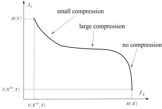
Figure 12.9: Regions of different types of compression on the information curve.
