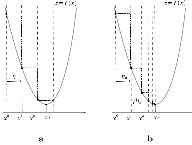
Figure 4.7: a. The use of a fixed learning rate \eta leads to missing the minimum x^* . b. An adjustable learning rate \eta_n provides a much better approximation of the minimum. In this case the descent amount is proportional with the slope of the curve at the respective points; these slopes become smaller as we approach the critical point x^* .
