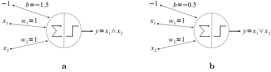
Figure 5.4: Boolean function implementation using a perceptron: a. The output function AND. b. The output function OR.
