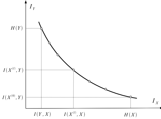
Figure 12.8: The information path associated with a neural network in the information plane.
