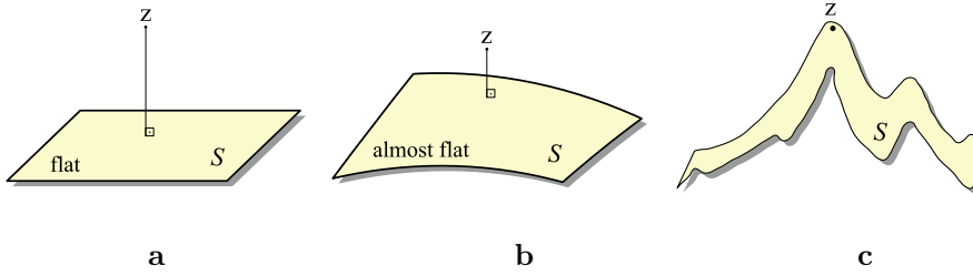
Figure 13.14: Regularization with a manifold \mathcal{S} of the same dimension but different degrees of flatness: (a) Using a plane leads to a large distance from the target \mathbf{z} , which underfits data; (b) using a trade-off between curvature and distance to \mathbf{z} leads to a good fit; (c) using a largely curved manifold we can always force the target point \mathbf{z} to belong to the manifold, case which corresponds to an overfit.
