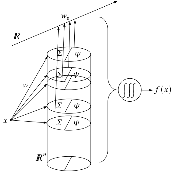
Figure 10.7: A one-hidden layer neural network with a continuum infinite number of computational units.
