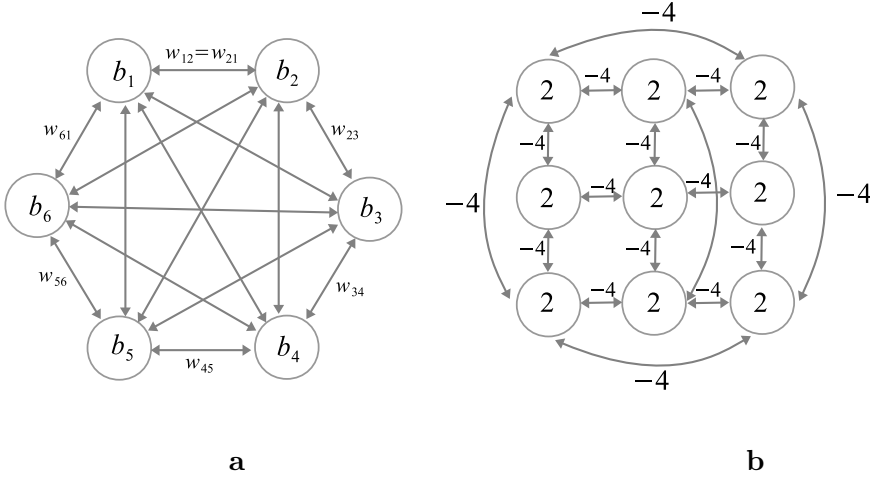
Figure 20.1: a A Hopfield network with n = 6 neurons; b . A Hopfield network associated with a 3 \times 3 chess board has nonzero connection weights only for vertically or horizontally connected units.
