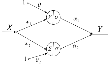
Figure 11.11: Network of two sigmoid neurons.
