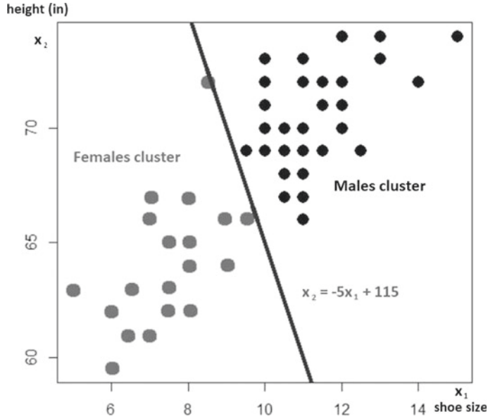
Figure 5.7: Perceptron classifying groups of males and females. The line x_2 = -5x_1 + 115 is a decision boundary in the feature space \{x_1, x_2\} between two linearly separable clusters.
