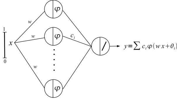
Figure 8.3: A one-hidden layer sigmoid neural network, with input to hidden layer weights w and hidden layer to output weights c_i .
