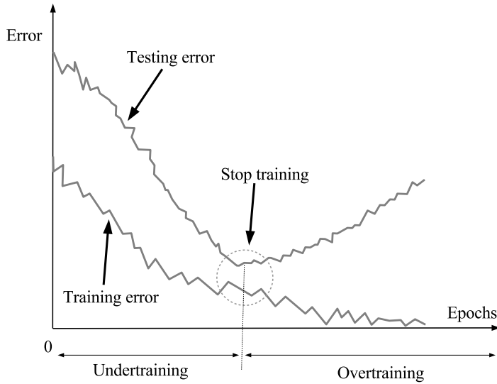
Figure 3.2: Overtraining and undertraining regions for a neural network. Since the training and testing errors are stochastic the optimal stopping is a random variable which is mostly contained in the dotted circle.
