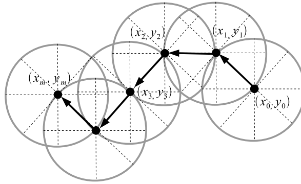
Figure 4.19: The search of the minimum starts at (x_0, y_0) and follows the arrows. At each step the point of the smallest values is chosen and a step into that direction is made.
