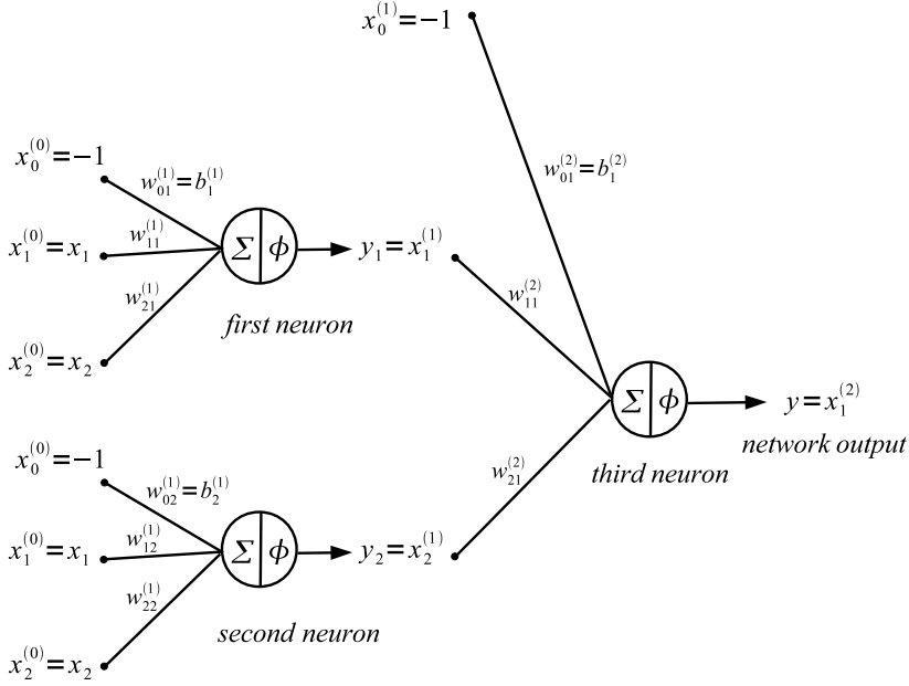
Figure 6.1: Two neurons with identical inputs, x_1, x_2 , and outputs y_1, y_2 , are fed into a third neuron with the output y .
