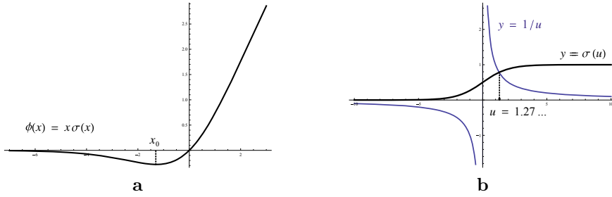
Figure 2.5: a. The activation function \phi(x) = x\sigma(x) has a minimum at the point x_0 \approx -1.27 . b. The graphical solution of the equation \sigma(x) = 1/x .
