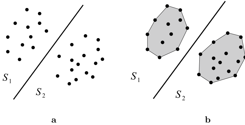
Figure 18.7: a. Linear separability of two clusters. b. Linear separability of the convex hulls of two clusters.
