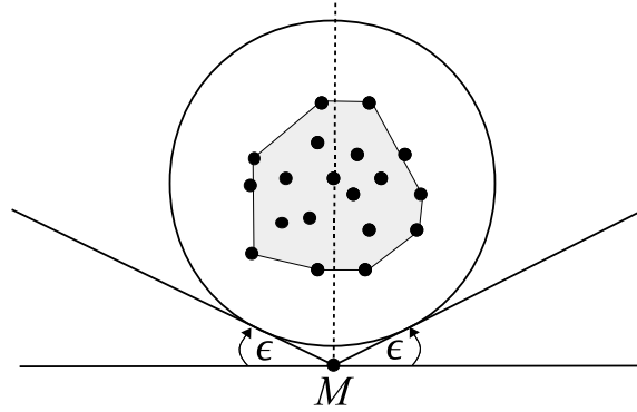
Figure 18.10: Construction of a disk that contains the convex hull of a cluster and is contained in a given half-plane.
