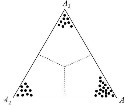
Figure 18.17: The dashed lines separate the triangle into three decision regions.
