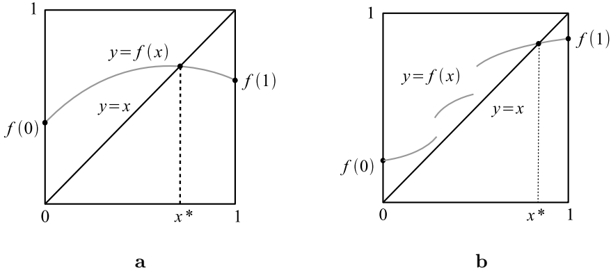
Figure 1: a. A fixed point of a continuous function f : [0, 1] \rightarrow [0, 1] . b. A fixed point of an increasing function f : [0, 1] \rightarrow [0, 1] .
