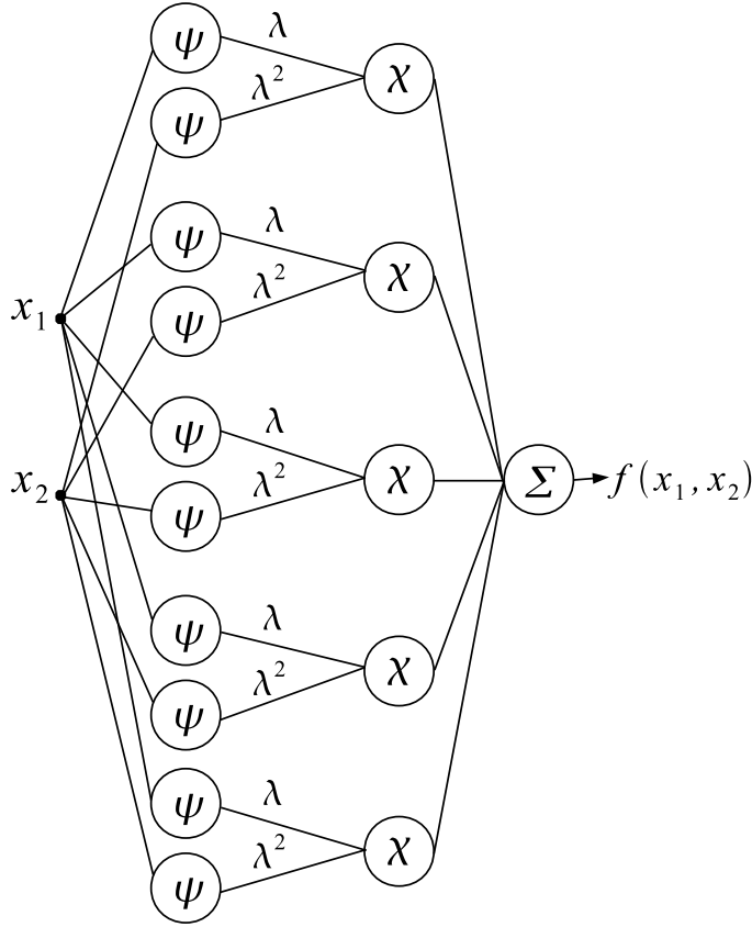
Figure 10.6: Two-hidden layer exact representation of a continuous function f in the case n = 2 .
