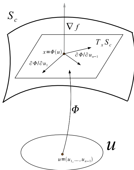
Figure 4.2: Local parametrization \Phi : \mathcal{U} \rightarrow \mathbb{R}^n of the hypersurface S_c .
