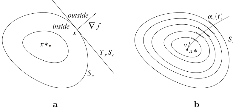
Figure 4.3: a. Gradient \nabla f normal to S_c . b. The curve \alpha_v(t) starting at x^* with initial velocity v .
