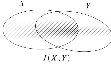
Figure 12.2: Each random variable is represented by a domain; the area of intersection of domains represents the mutual information I(X, Y) .
