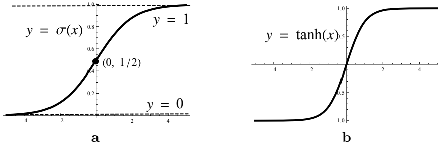
Figure 2.8: a. Logistic function \sigma(x) = \frac{1}{1+e^{-x}} and its horizontal asymptotes, y = 0 and y = 1 . b. Hyperbolic tangent function.
