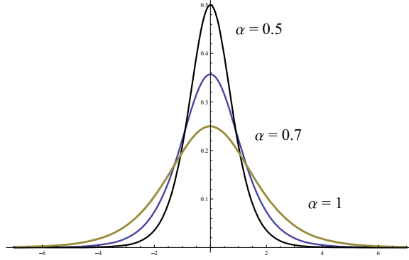
Figure 8.8: The convolutional kernels K_\alpha(x) converge to a “spike” centered at zero, as \alpha \rightarrow 0 .
