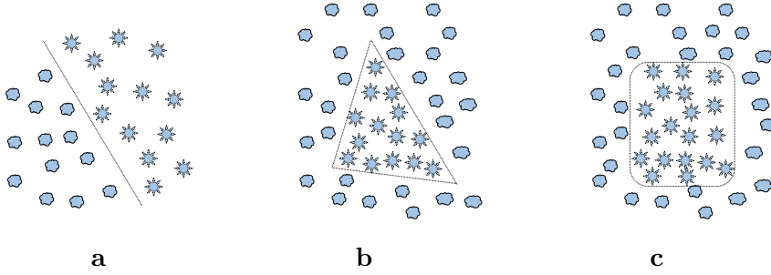
Figure 11.13: a. The clusters can be separated by a line; b. One cluster is inside of a triangle and the other is outside; c. One cluster lies inside of a rectangle.
