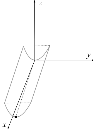
Figure 4.8: The graph of z = \frac{1}{2}y^2 - x .
