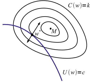
Figure 3.3: The cost function C(w, b) has a minimum at point M ; its level surfaces are given by \mathcal{S}_k = \{C(w, b) = k\} . One of these level surfaces is tangent to the surface \{U(w) = c\} at a point where the gradients \nabla C and \nabla U are collinear.
