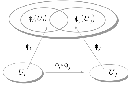
Figure 13.1: The transitions functions \phi_i \circ \phi_j^{-1} of a manifold are differentiable.
