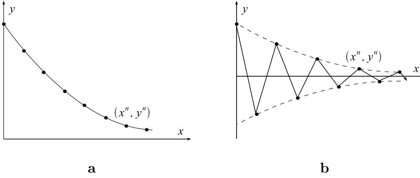
Figure 4.9: Iterations: a. Case 0 < \delta < 1 . b. Case 1 < \delta < 2 .
