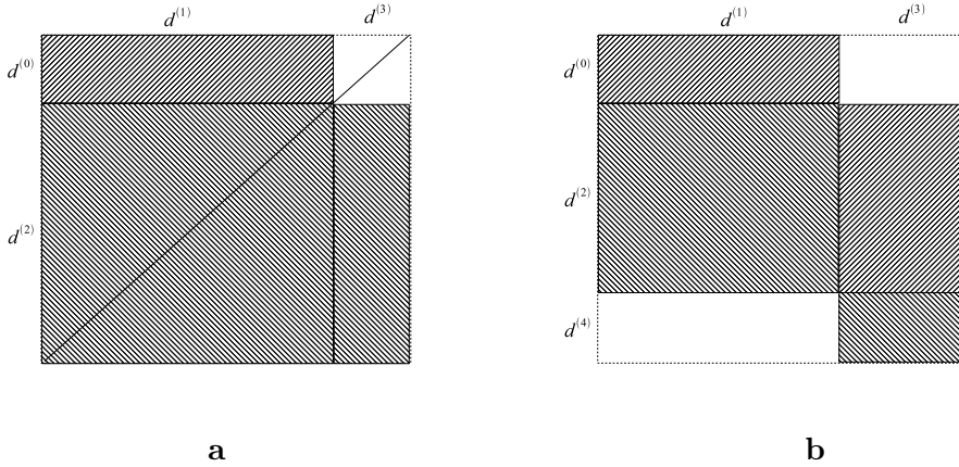
Figure 13.9: a. The blank rectangle is a square of area d^{(0)}d^{(3)} = 1 . b. The blank rectangles have an area larger than 1.
