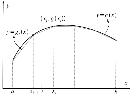
Figure 8.6: The polygonal line g_\epsilon(x) converges uniformly on [a, b] to the continuous function g(x) , as \epsilon \rightarrow 0 .
