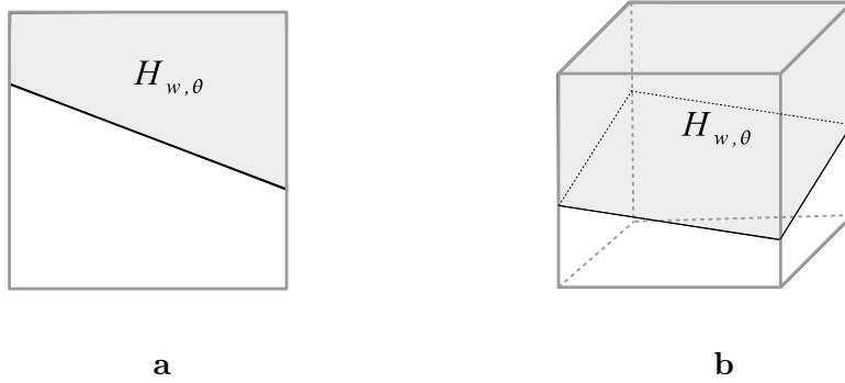
Figure 9.3: The upper half-space for: a. the unit square I_2 . b. the unit cube I_3 .
