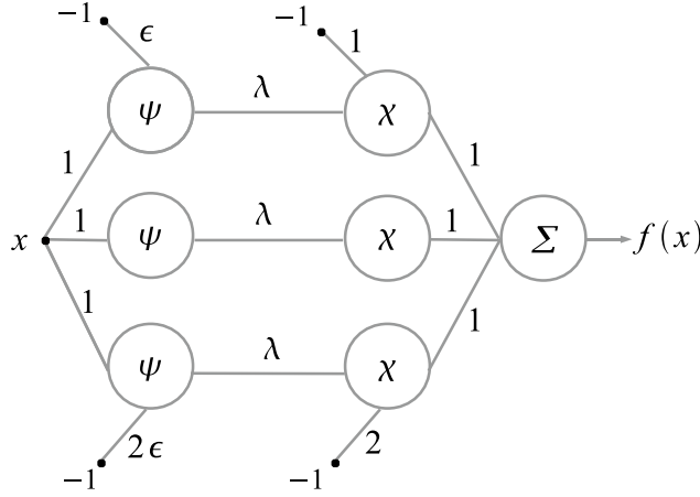
Figure 10.5: Two-hidden layer exact representation of a continuous function f in the case n = 1 .
