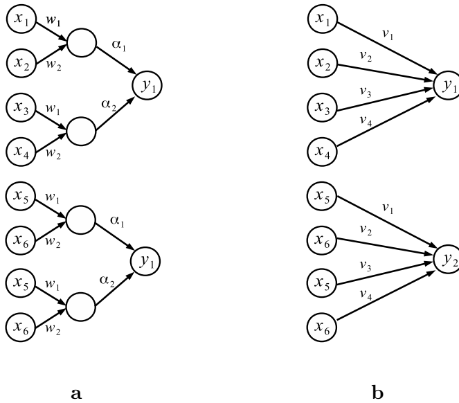
Figure 16.4: Two equivalent convolutional networks: a one-hidden layer convolutional net with stride equal to 2; b two-layer convolutional net with stride equal to 4.
