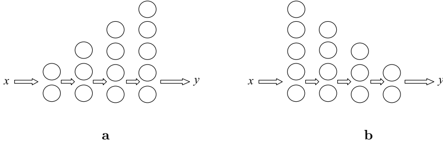
Figure 13.11: Two symmetric networks, which depend on the same number of parameters: a. An encoder. b. A decoder. The number of parameters is 59; there are 14 biases (one for each neuron) and 45 weights.
