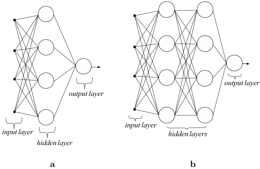
Figure 6.5: a. One-hidden layer neural network; b. Two-hidden layer neural network.
