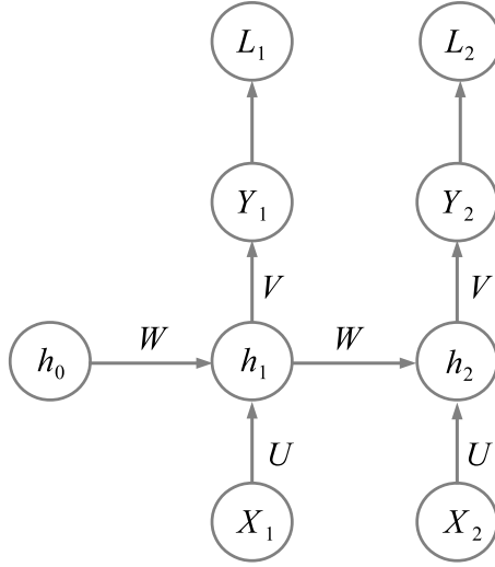
Figure 17.3: An RNN configuration with two steps.
