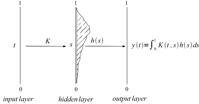
Figure 10.8: A three-layer neural net with a continuum of neurons in the hidden layer.
