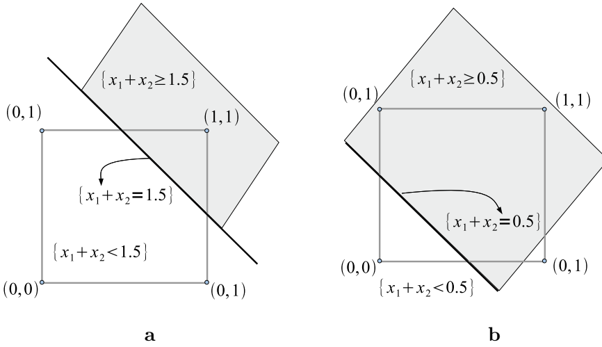
Figure 5.5: Partition using a perceptron; the shaded half-plane is associated the value 1. a. The output function AND. b. The output function OR.
