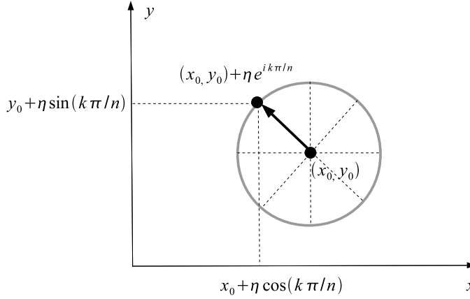
Figure 4.18: The circle of center (x_0, y_0) and radius \eta is divided into n equal sectors. At each step the point of the smallest value is chosen and a step into that direction is made.
