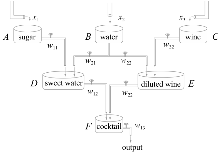
Figure 1.10: A cocktail factory as a neural network with two hidden layers.
