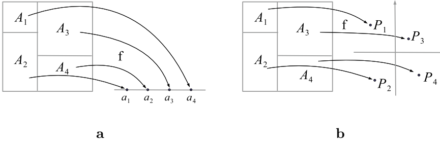
Figure 18.4: Decision map associated with a partition: a. The label space is \mathbb{R} . b. The label space is \mathbb{R}^2 .
