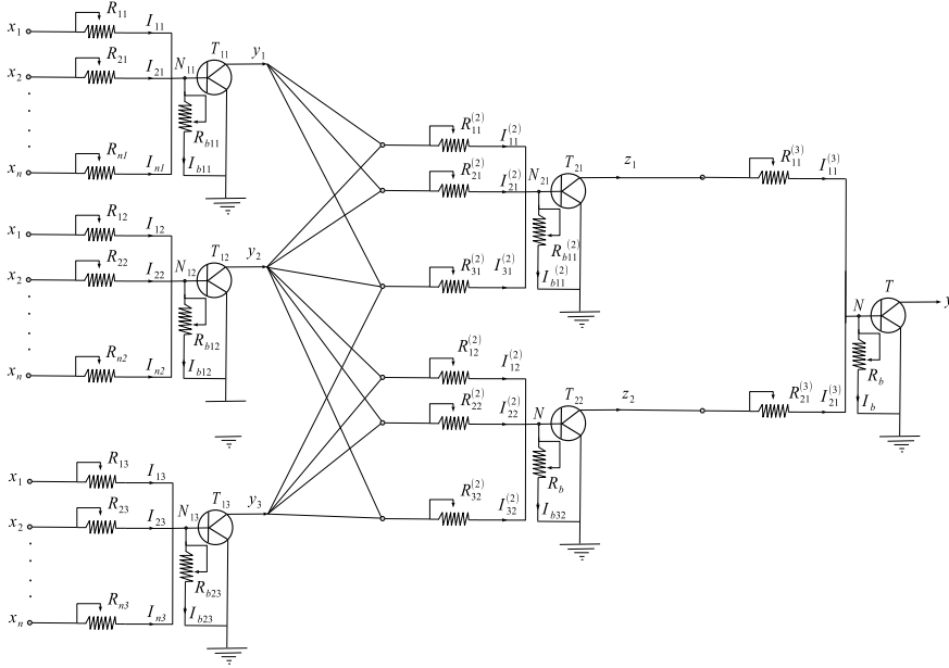
Figure 1.11: Neural network with two hidden layers and 6 transistors. Each transistor implements a logic gate.
