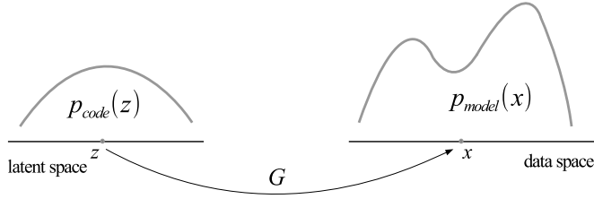
Figure 19.1: The transformation G between the latent space and data space.
