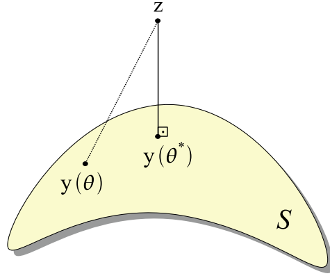
Figure 13.10: The orthogonal projection of \mathbf{z} on the manifold \mathcal{S} is \mathbf{y}(\theta^*) .
