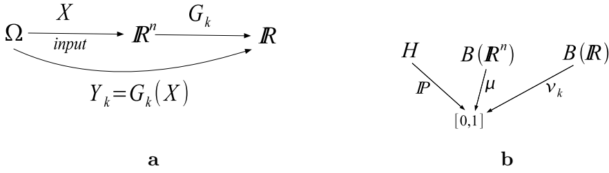
Figure 11.5: a. The estimations Y_k . b. The distribution measures \nu_k of Y_k .
