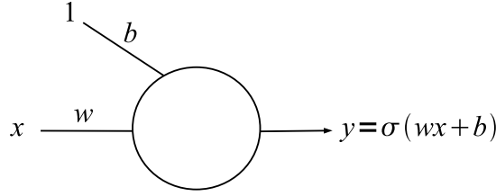
Figure 13.15: The manifold \mathcal{S} associated with a sigmoid neuron is 2-dimensional.
