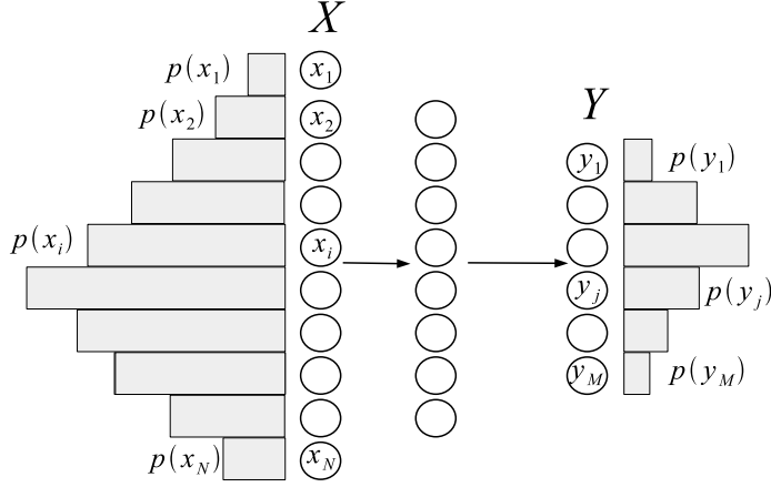
Figure 12.6: The output density p(y_j) in terms of the input density p(x_i) .
