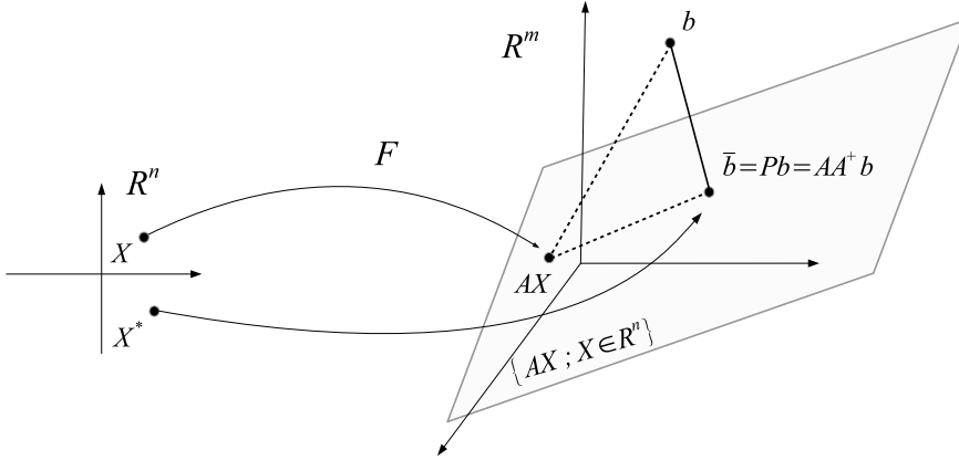
Figure 1: The geometric interpretation of the pseudoinverse solution X^* = A^+b .
