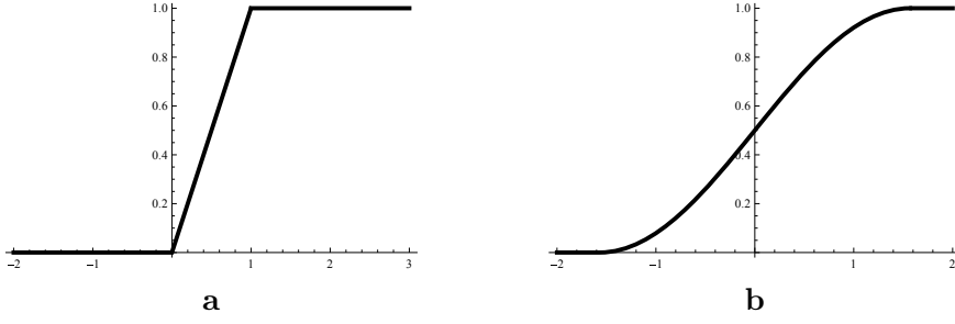
Figure 2.11: Squashing functions: a. Ramp function b. Cosine squasher function.
