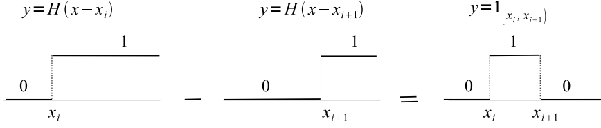
Figure 8.1: The indicator function as a difference of two Heaviside functions, 1_{[x_i, x_{i+1})}(x) = H(x - x_i) - H(x - x_{i+1}) .
