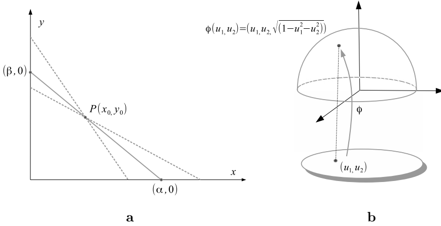
Figure 13.2: a. The manifold of lines passing through the point P(x_0, y_0) and their axes intercepts. b. The upper half-sphere.
