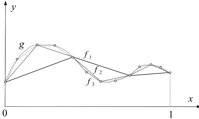
Figure 7.2: A polygonal approximating sequence (f_n)_n satisfying the inequality |g(x) - f_{n+1}(x)| \leq |g(x) - f_n(x)| , for all x \in [0, 1] .
