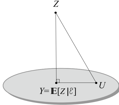
Figure 3.1: The best predictor of the target Z , given the information \mathcal{E} , is the orthogonal projection of Z on the space of \mathcal{E} -measurable functions.
