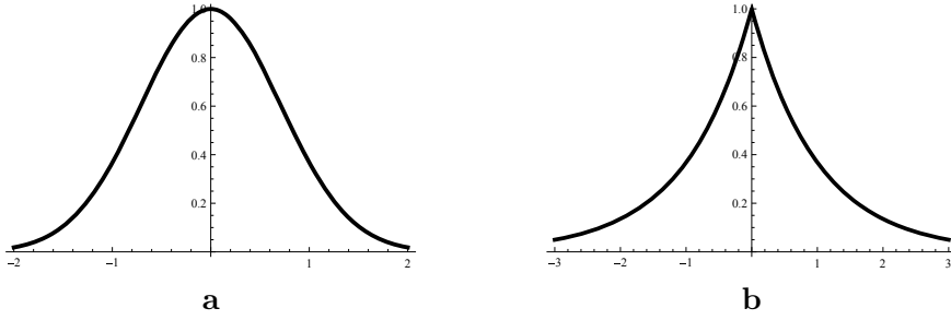
Figure 2.10: a. Gaussian function g(x) = e^{-x^2} b. Double exponential function f(x) = e^{-|x|} .
