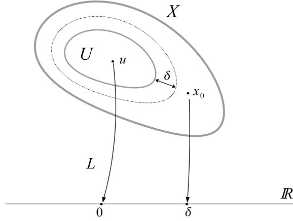
Figure 9.1: The functional L that vanishes on subspace \mathcal{U} , see Lemma 9.3.1.
