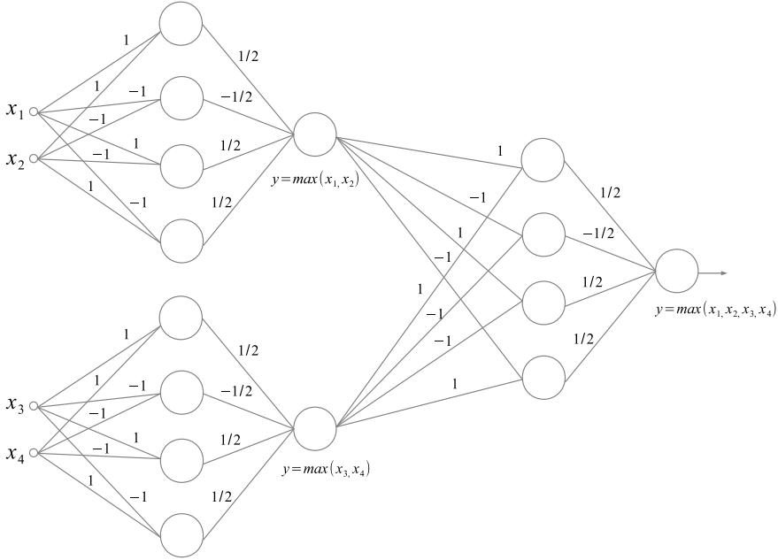
Figure 10.2: A neural network learning exactly the maximum of 4 numbers. The 8 neurons in the first layer can be considered as only 4 overlaying neurons.
