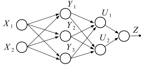
Figure 1: In a feedforward neural network the information flow satisfies the sequence of inclusions \mathcal{F}_Z \subset \mathcal{F}_U \subset \mathcal{F}_Y \subset \mathcal{F}_X , which forms a filtration.
