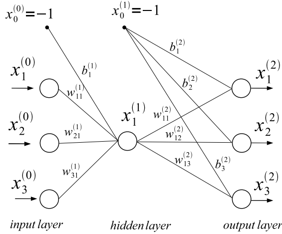
Figure 12.1: Autoencoder with one hidden neuron.
