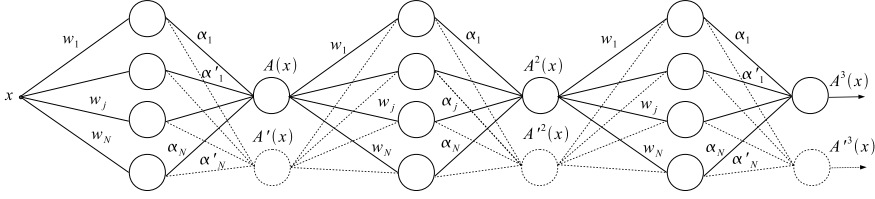
Figure 7.6: A recurrent neural net constructed from two \epsilon -close three-layer neural units.
