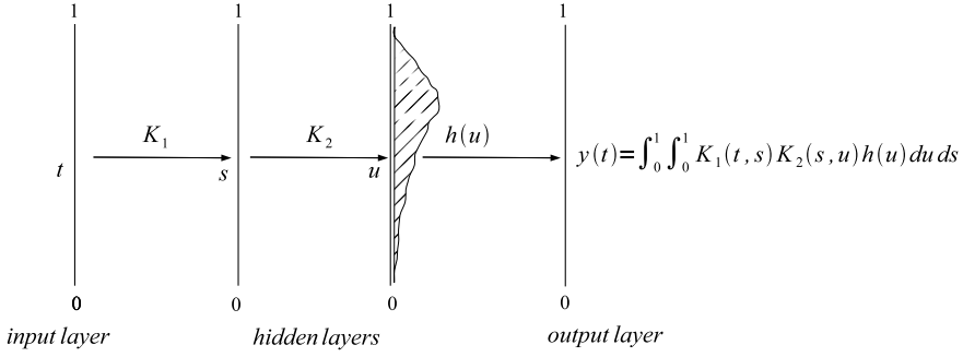
Figure 10.9: A four-layer neural net with a continuum of neurons in each hidden layer.
