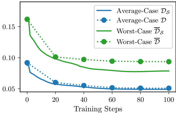
Distinguishability Loss
