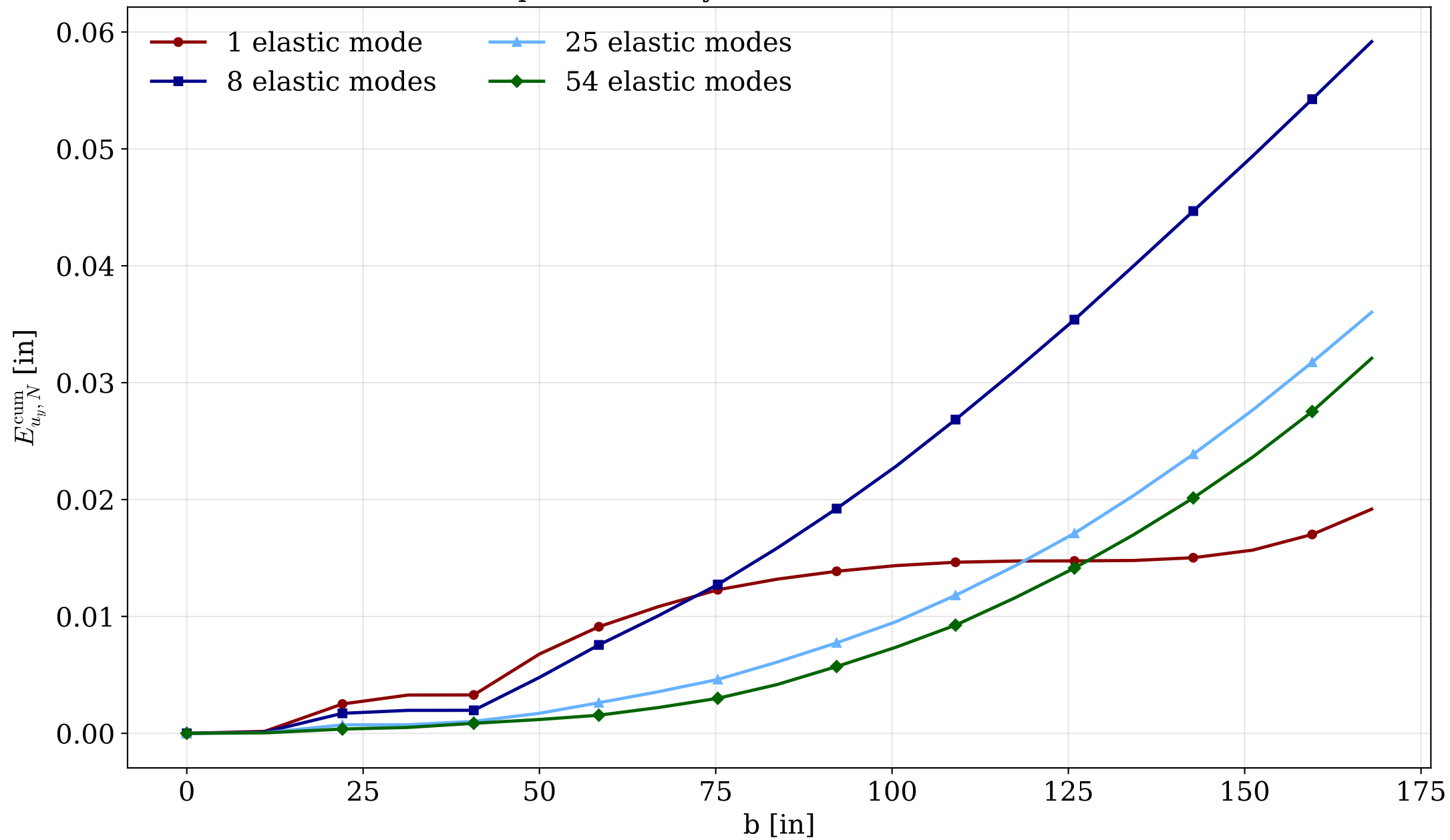
Displacement in y direction cumulative error
