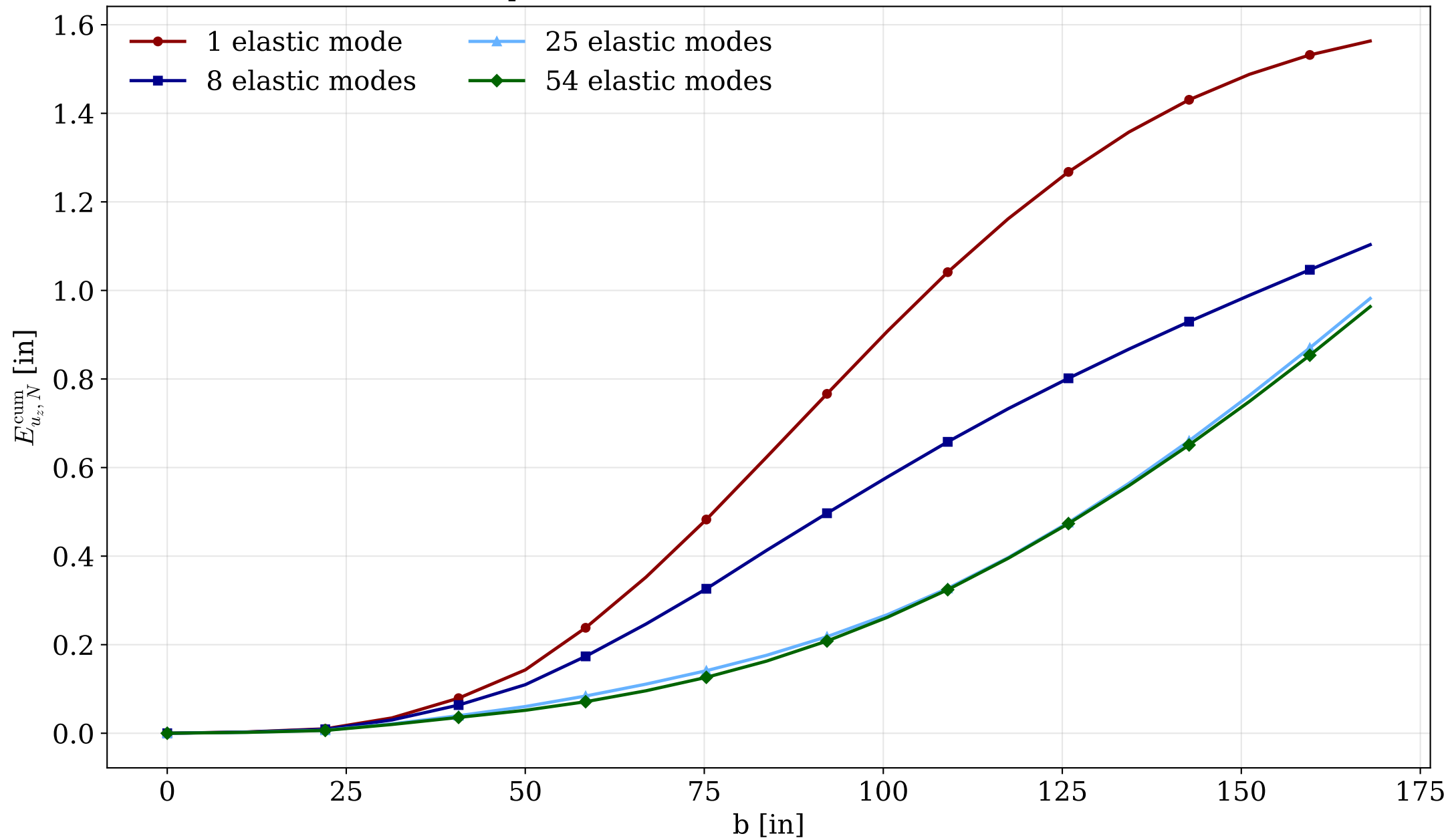
Displacement in z direction cumulative error
