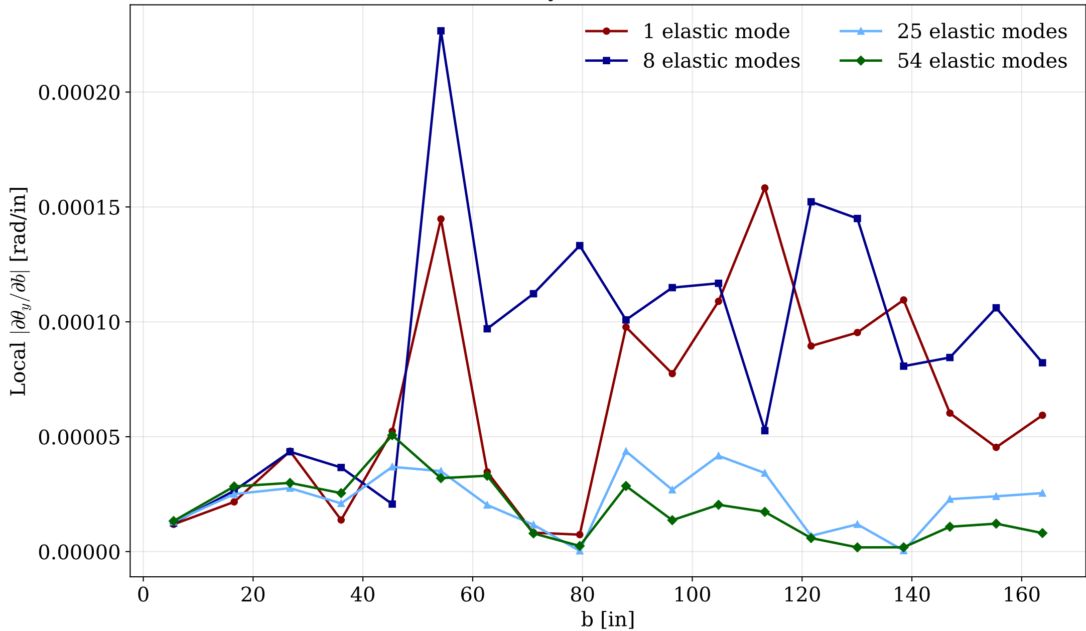
Rotation about y axis local curvature error
