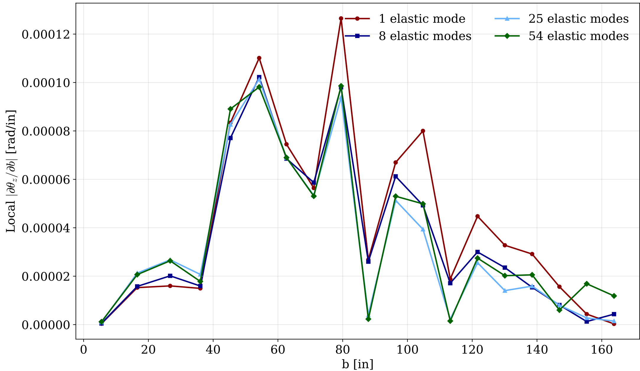
Rotation about z axis local curvature error
