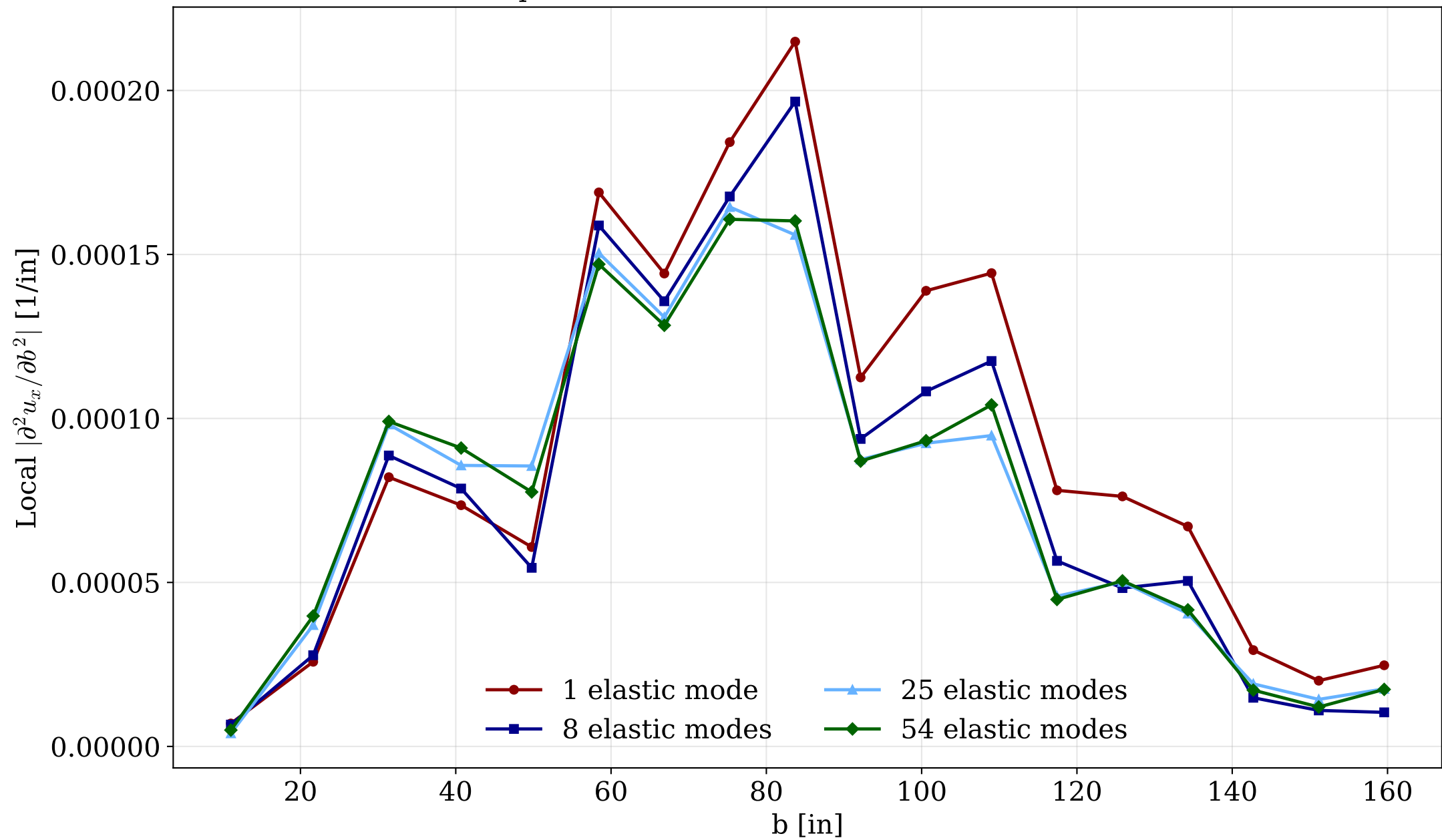
Displacement in x direction local curvature error
