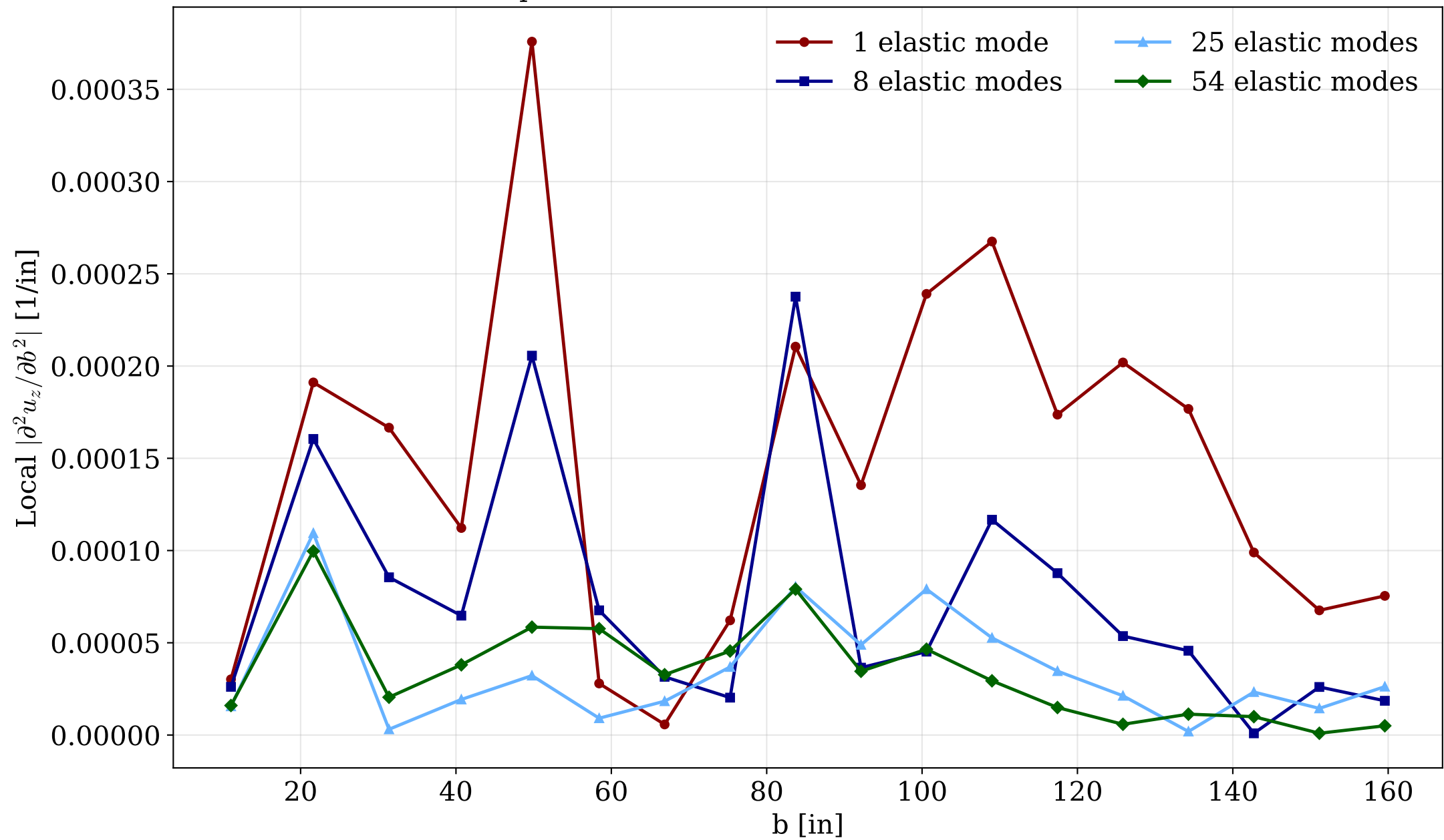
Displacement in z direction local curvature error
