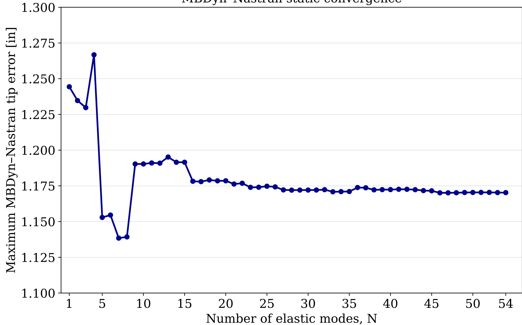
MBDyn-Nastran static convergence
