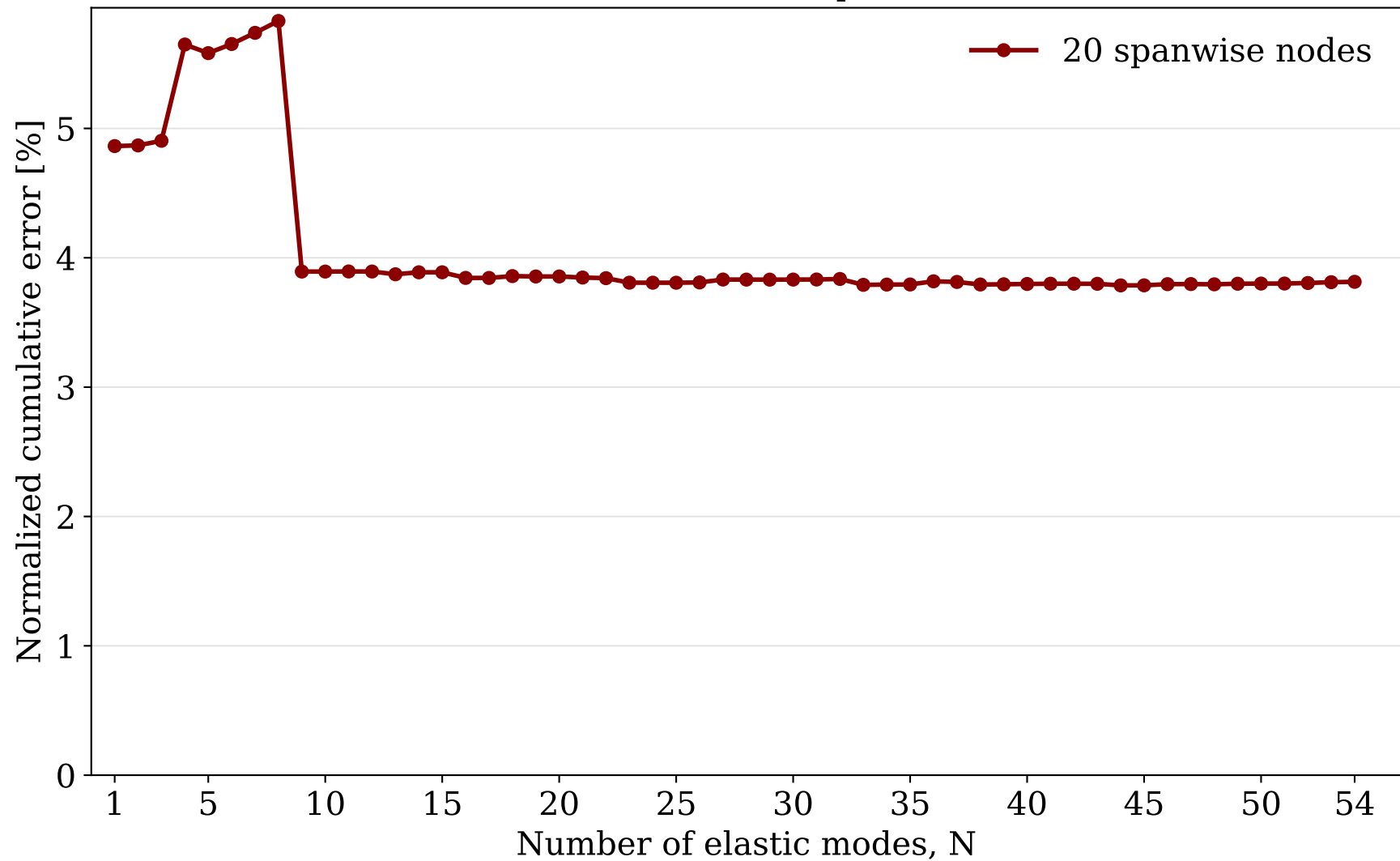
Normalized cumulative spanwise error
