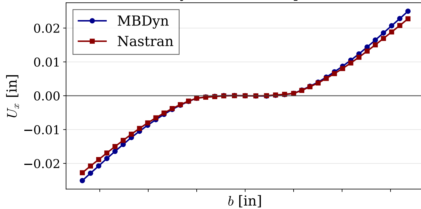
MBDyn-Nastran comparison
