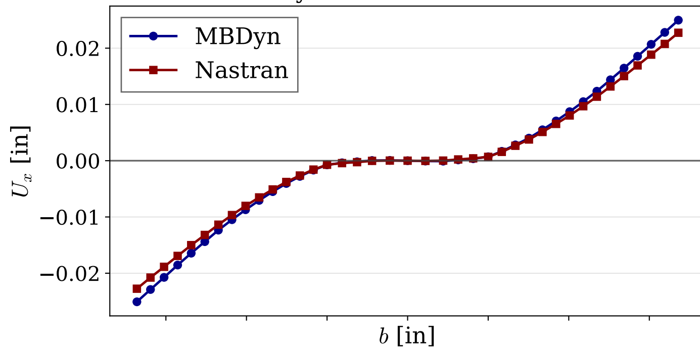
MBDyn-Nastran deformation
