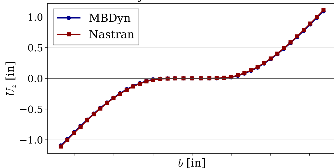
MBDyn-Nastran deformation
