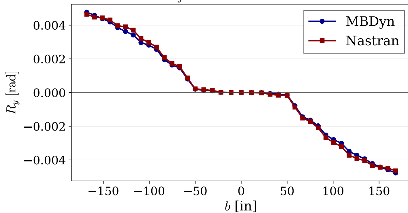
MBDyn-Nastran deformation
