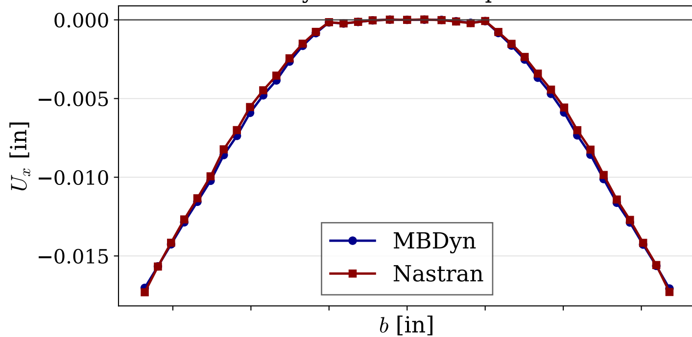
MBDyn-Nastran comparison
