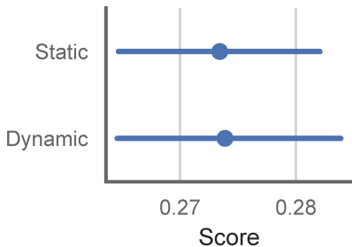
IFBench
