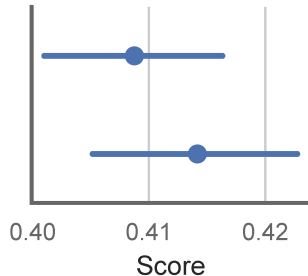
MATH
