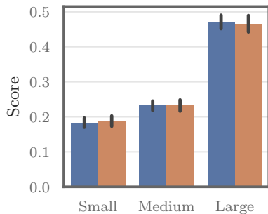
IFBench
