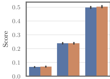
IFBench
