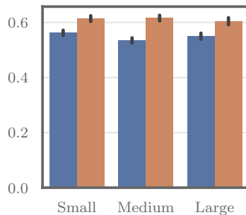
FLORES+
