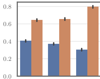
FLORES+
