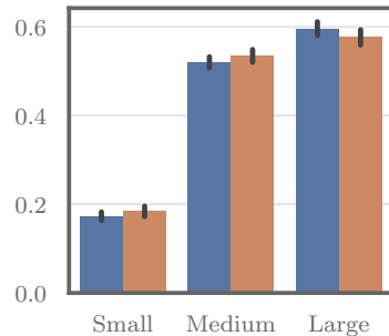
MATH
