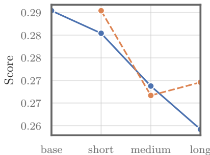
IFBench
