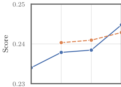
IFBench
