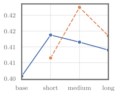
MATH
