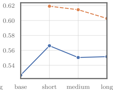
FLORES+
