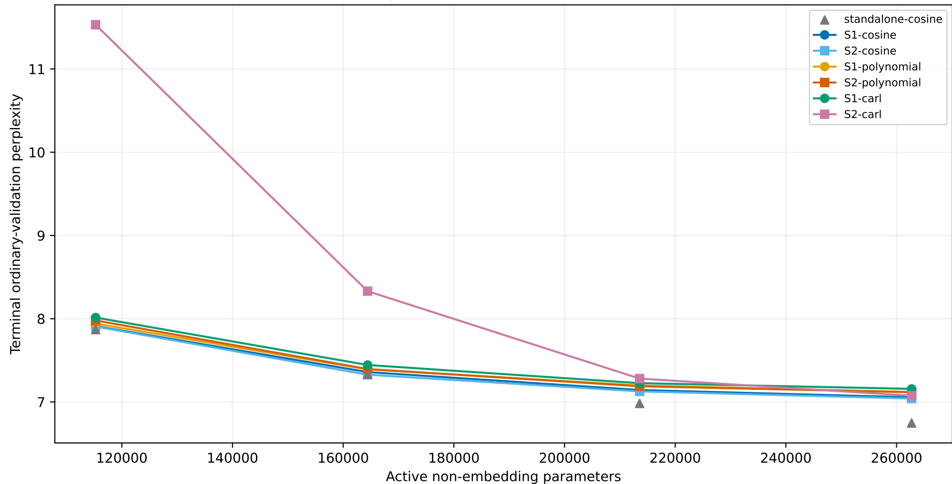
TinyStories-Instruct · linear widths
