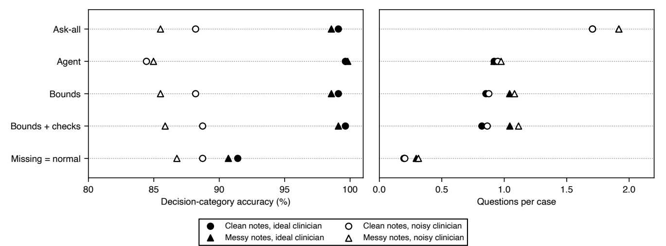
Figure 2: Decision-category accuracy (left) and questions per case (right) for each policy under the four conditions (Haiku extraction, 559 cases with validated notes in both styles). Symbols that coincide overlap: for example, ask-all asks the same questions whichever clinician answers
