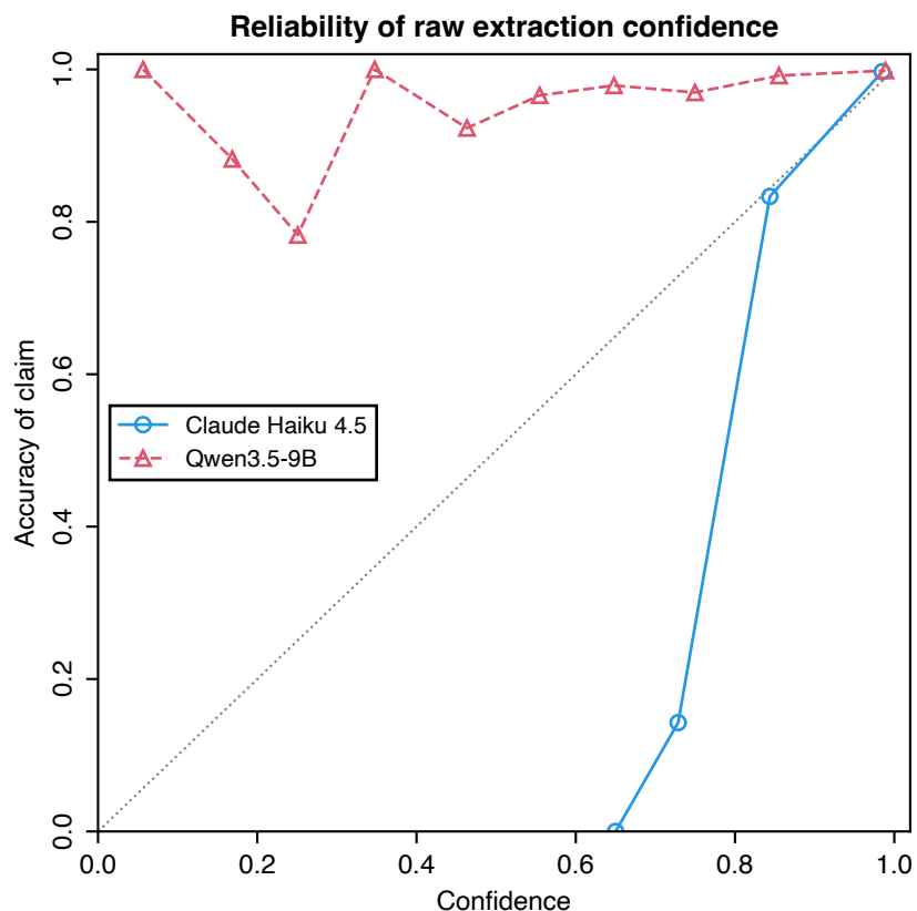
Figure 1: Reliability of raw extraction confidence (test split).
