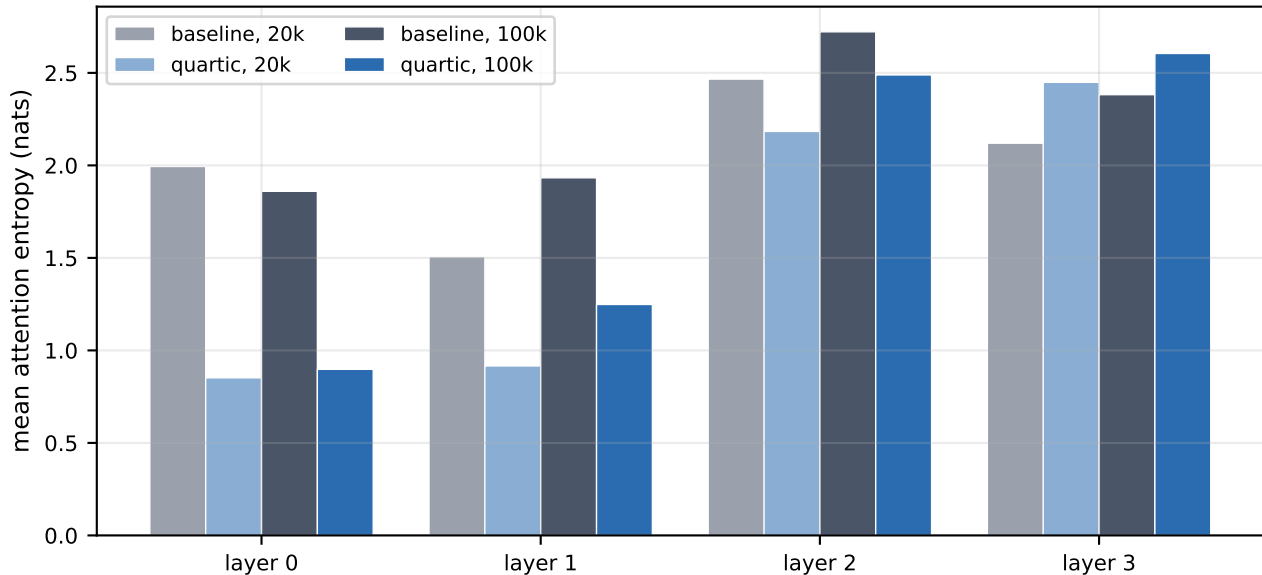
What the constraint leaves behind early-layer entropy stays low at 5× longer training
