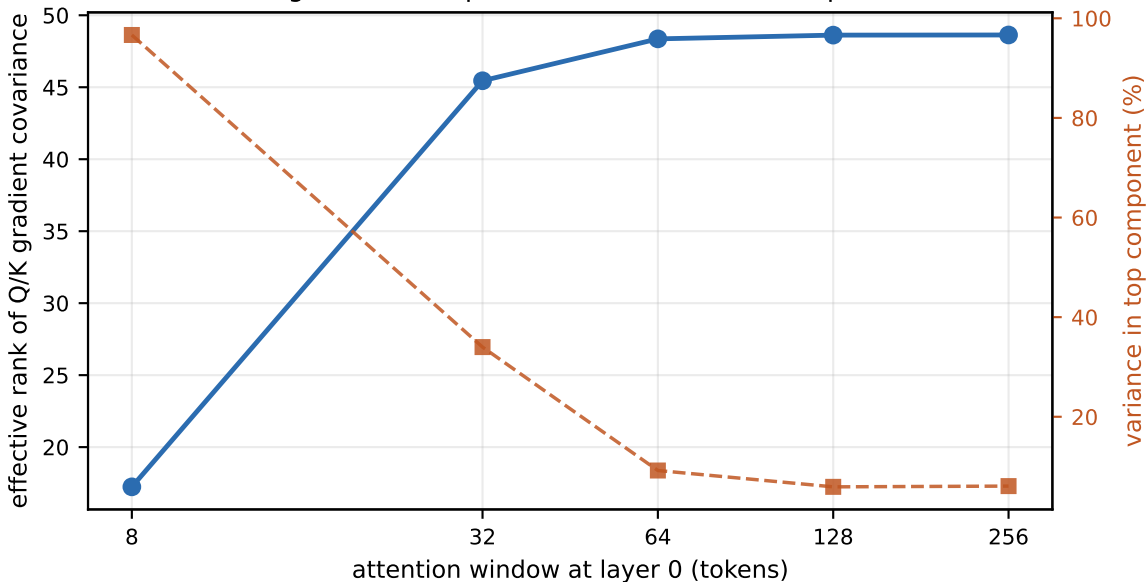
The constraint makes early updates coherent 50 gradient samples, frozen baseline checkpoint
