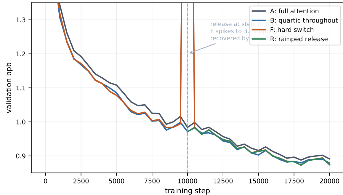
Removal at the halfway point, seed 137 legacy harness (training-time curves)
