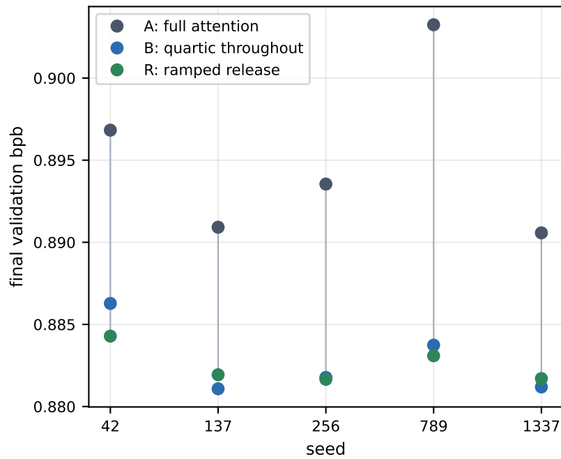
Paired endpoints, all five seeds (fixed harness)
