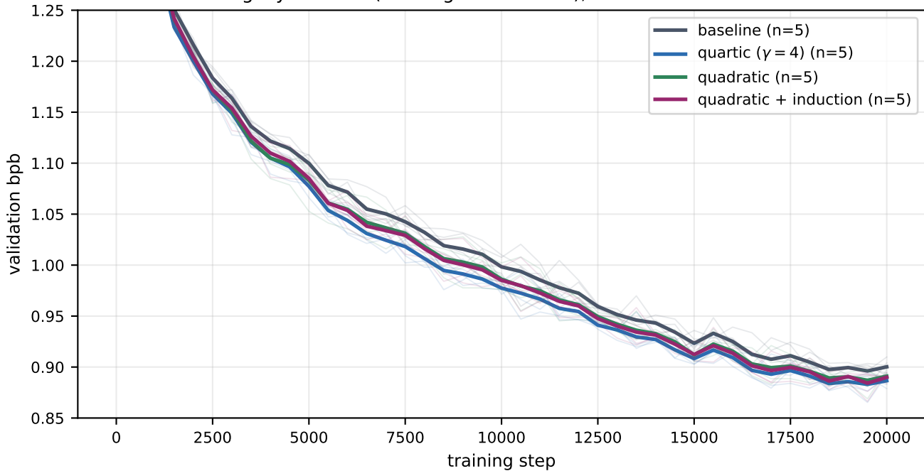
3.4M window variants, 20k steps, five matched seeds legacy harness (training-time curves); thin lines are seeds
