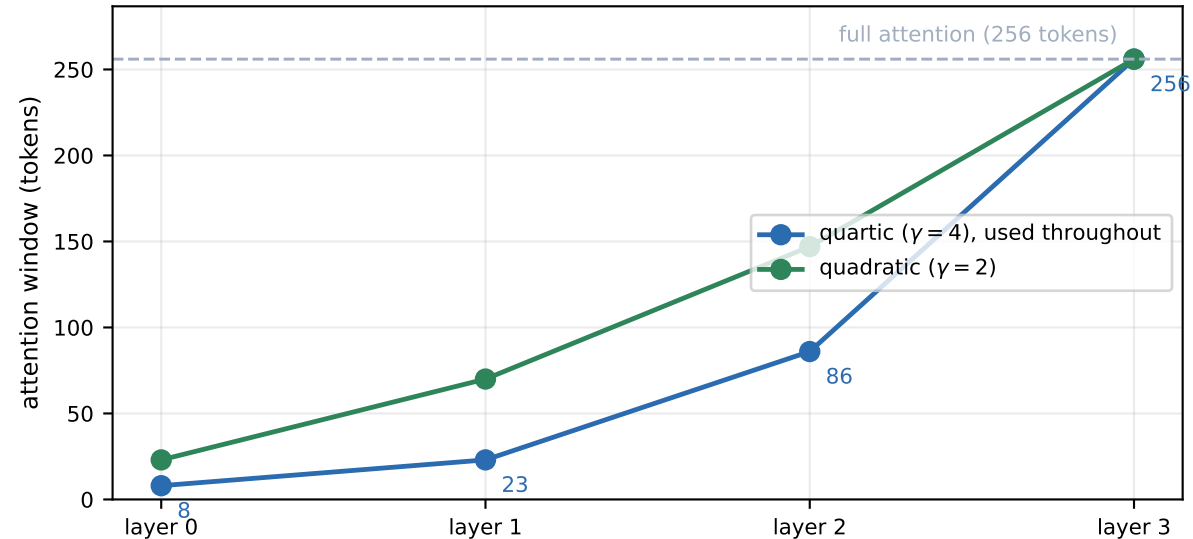
Depth-wise window schedule at depth 4, sequence length 256 early layers see a short span, the last sees everything
