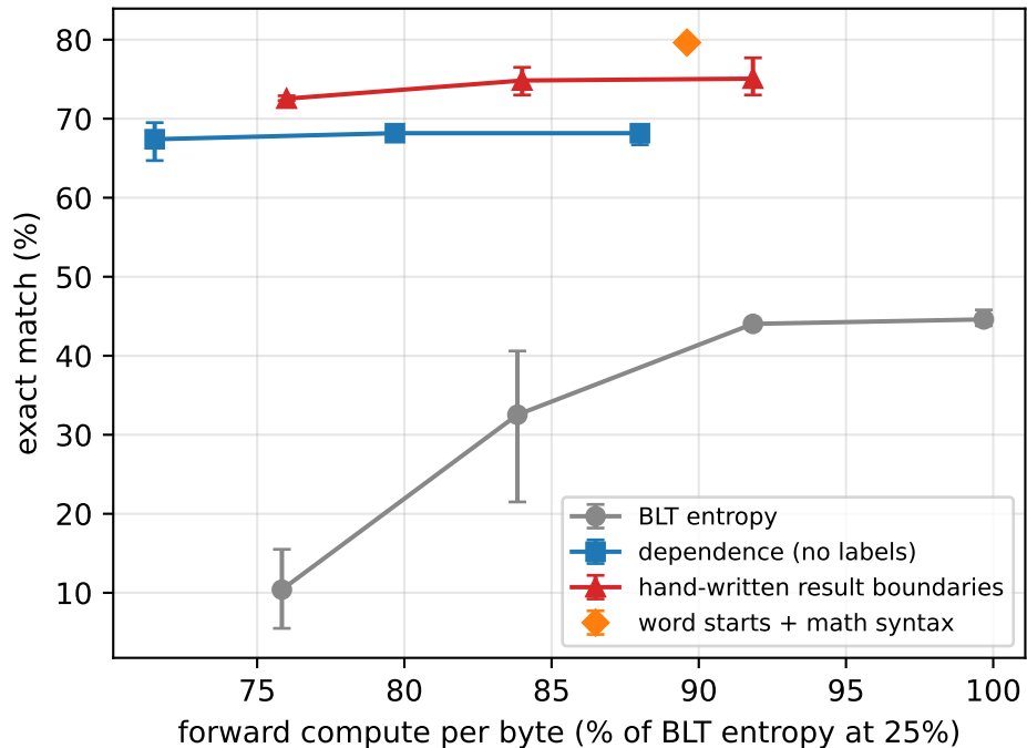
Final answers (GSM8K)
